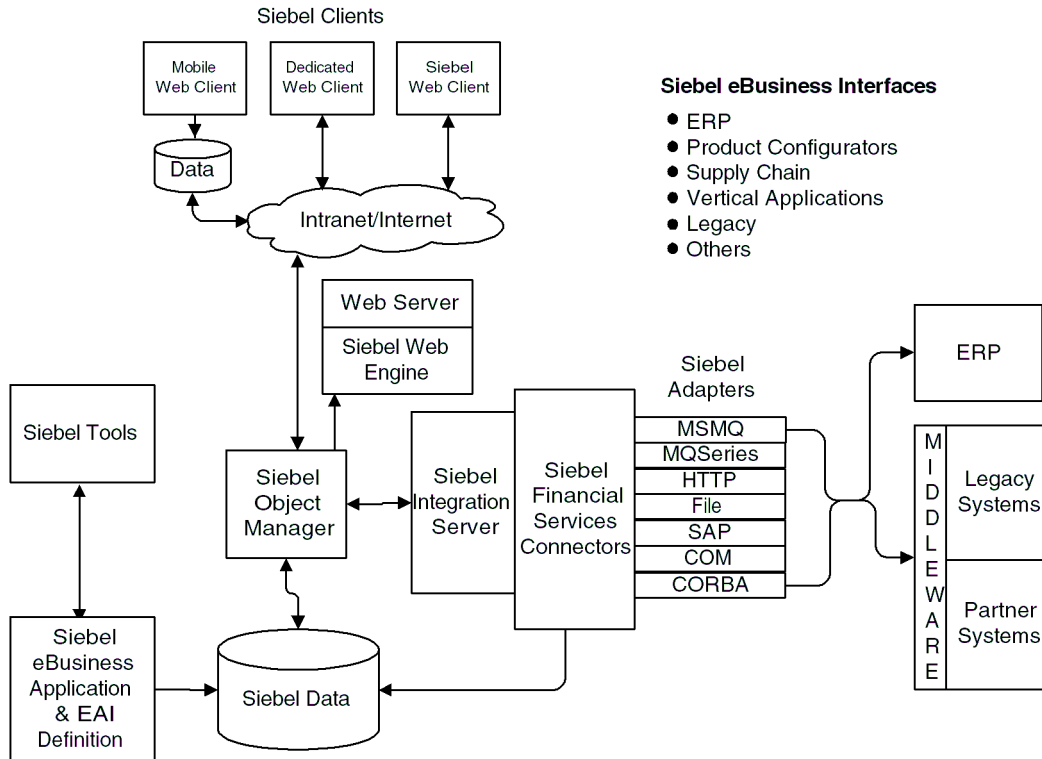
Figure 7. Siebel eBusiness Interfaces
