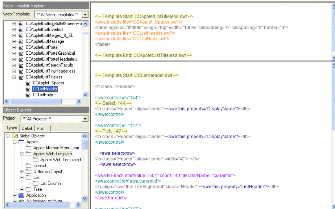
Figure 12. Example of Web Template Explorer Window with HTML Code Window
