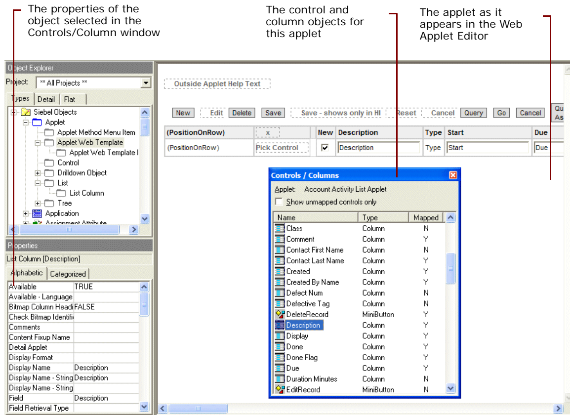
Figure 10. Example of the Controls/Columns Window with the Web Applet Editor
