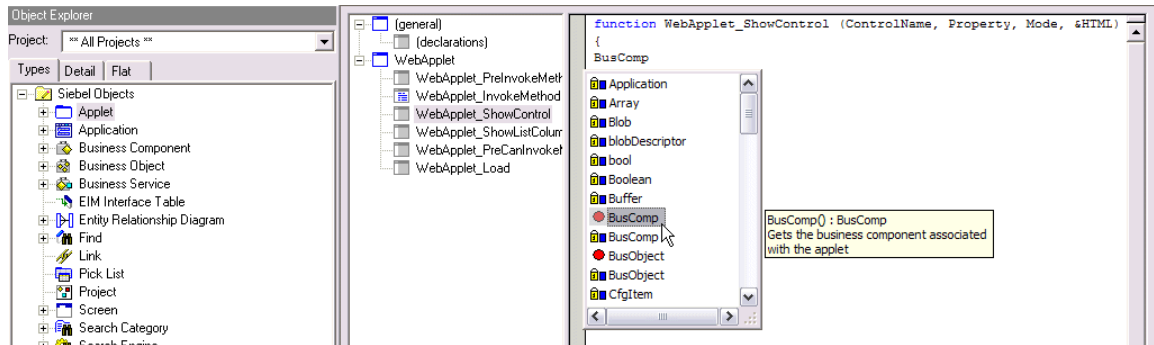
Figure 22. Method List
