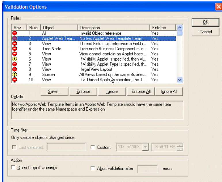
Figure 17. Validation Options Dialog Box
