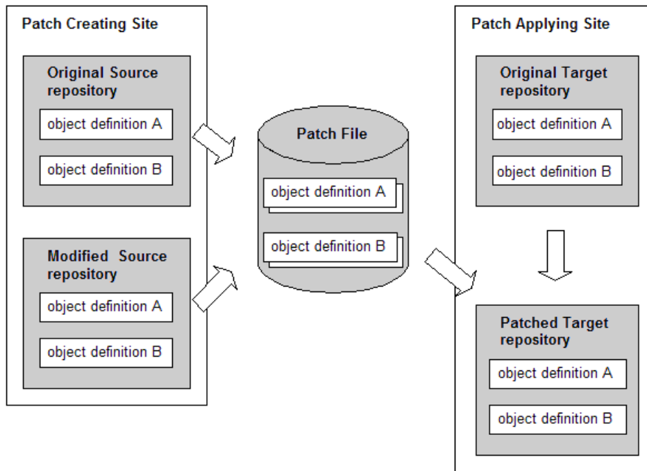
Figure 24. How a Patch Works
