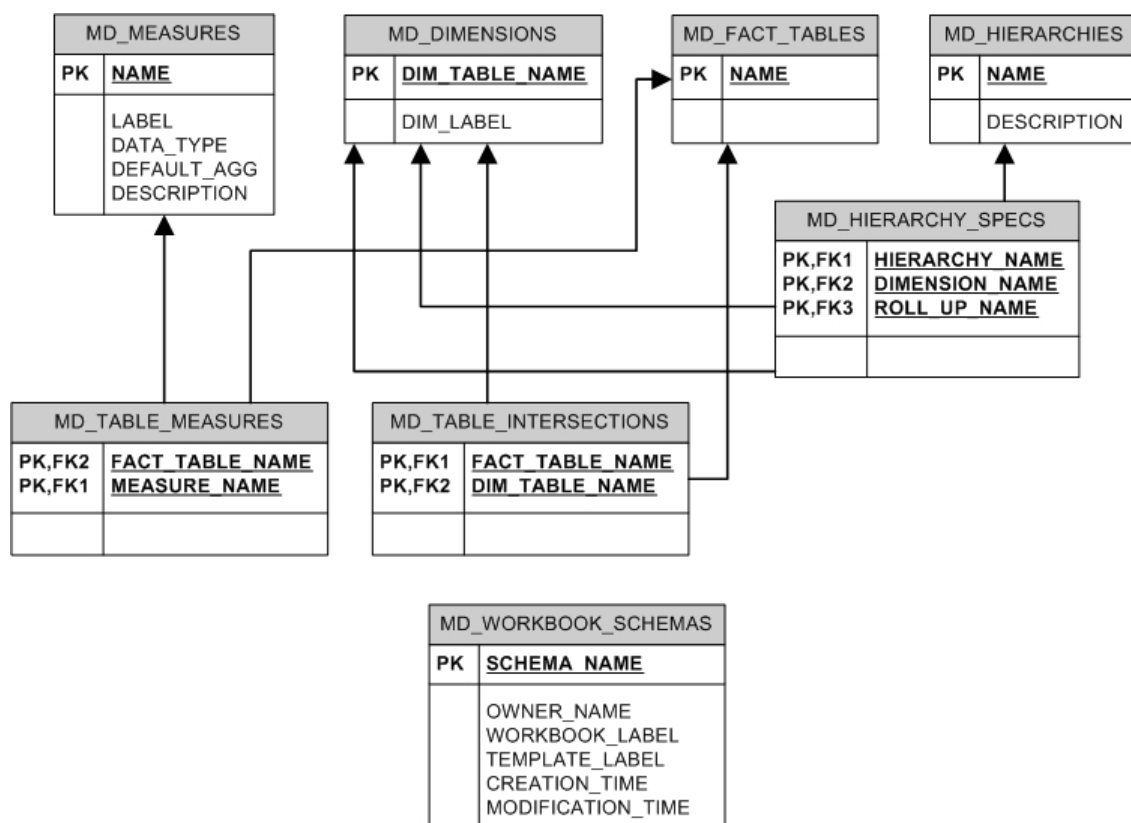
Figure 1: Database diagram for all metadata tables in a domain or in each workbook.
