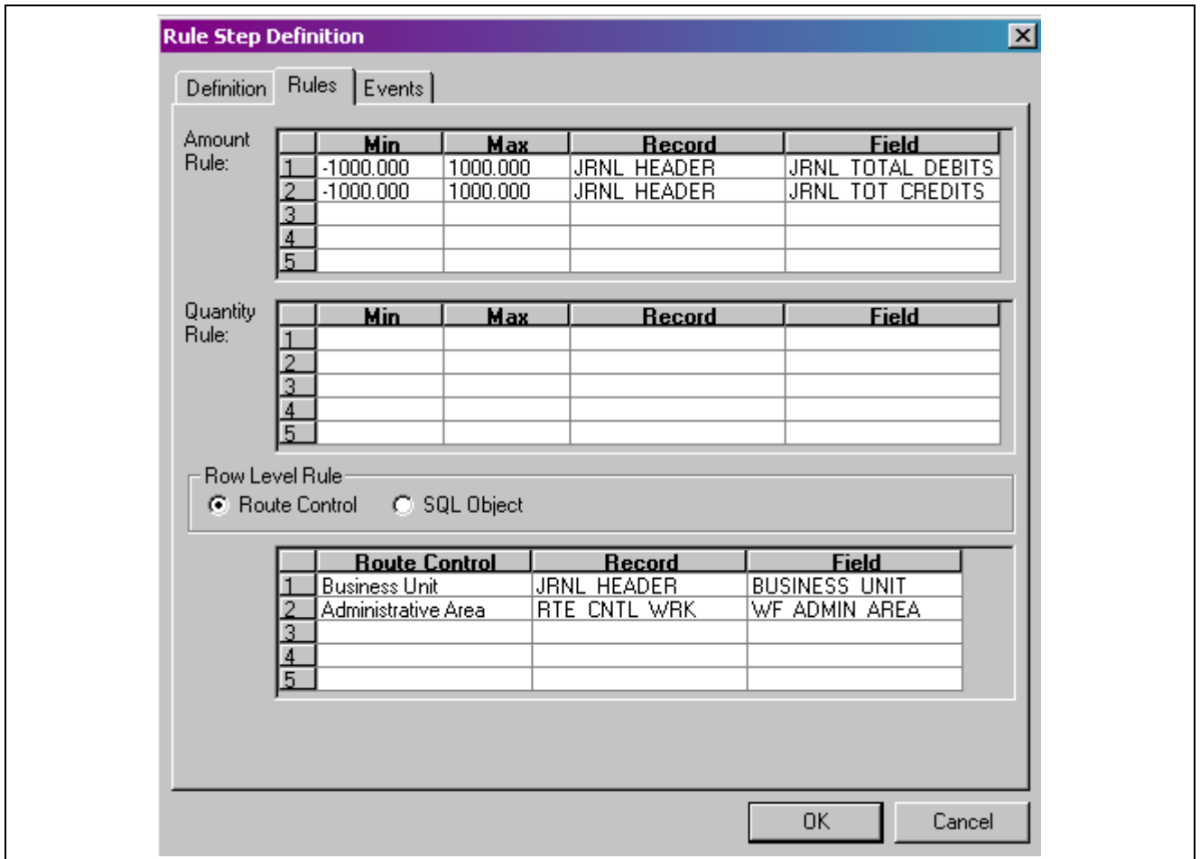
Rule Step Definition - Rules tab
