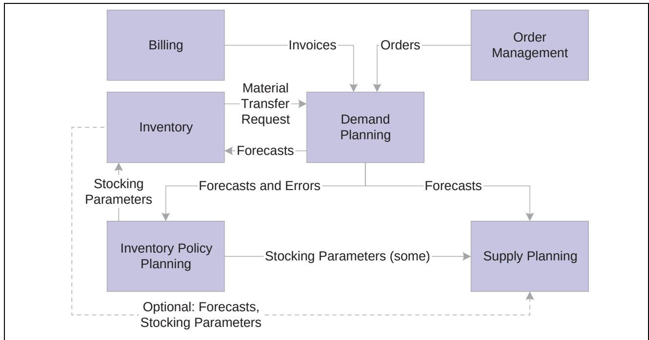
PeopleSoft Inventory Policy Planning integration points
