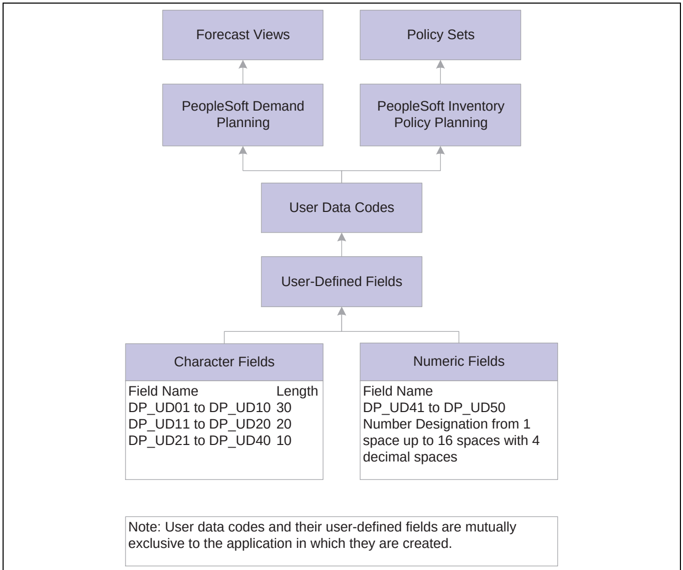
User data code relationships with policy sets and forecast views
