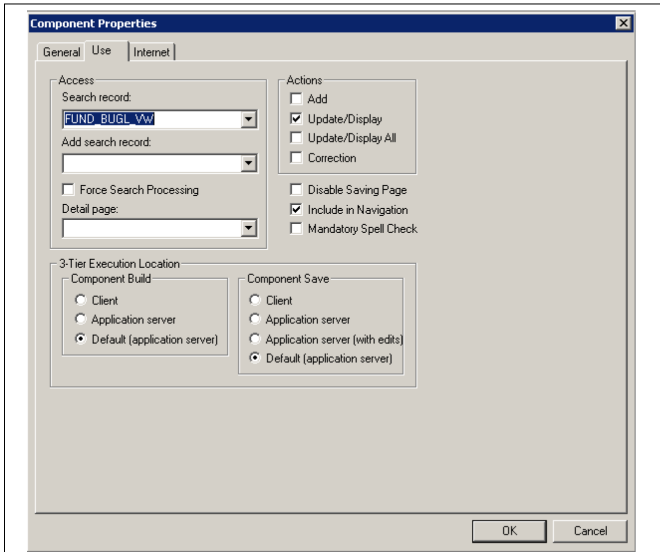
Component Properties page: Use tab
