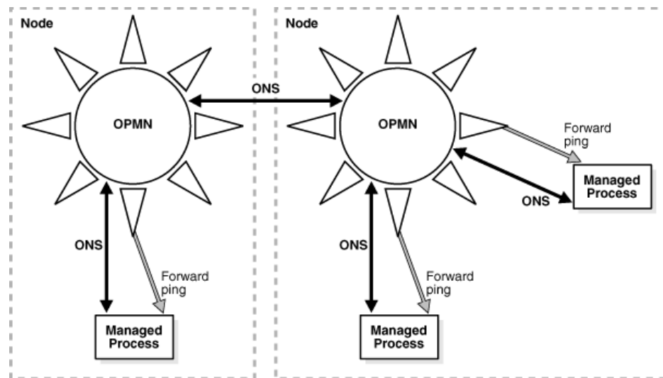
Figure 2–2 Process Management on Two Nodes
