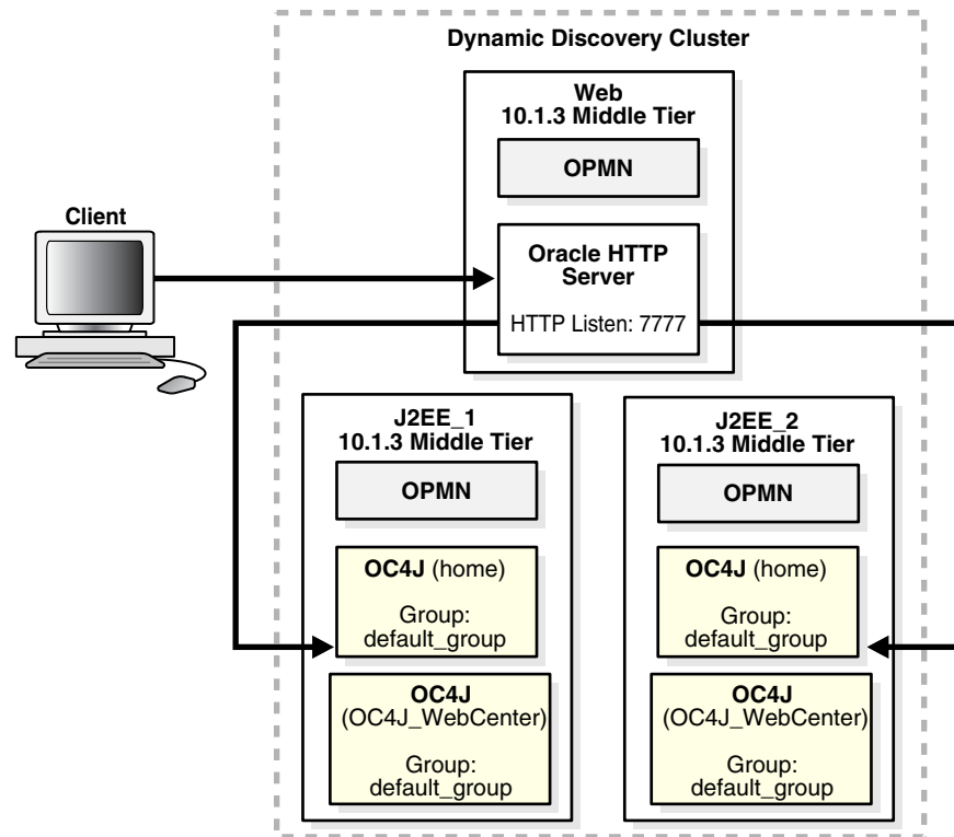
Figure 6–6 Multiple J2EE Server Middle Tiers and a Web Server Middle Tier in a Cluster
