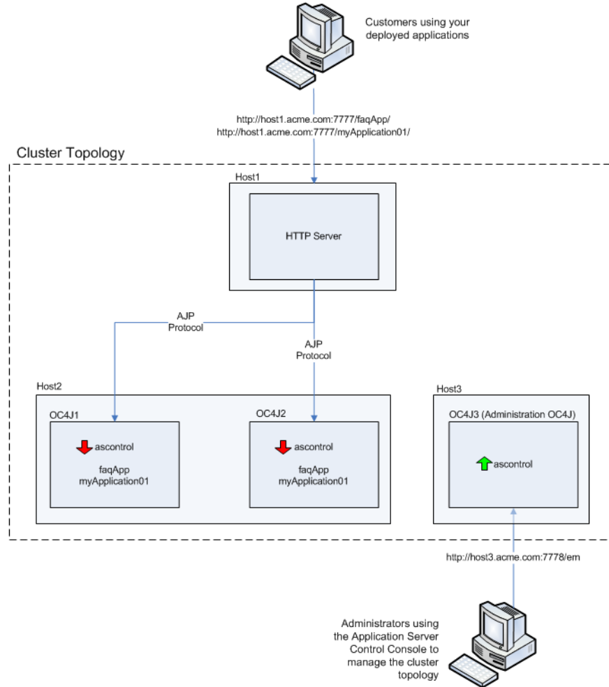
Figure A-3 Managing the Cluster Topology Using the Administration OC4J HTTP Listener
