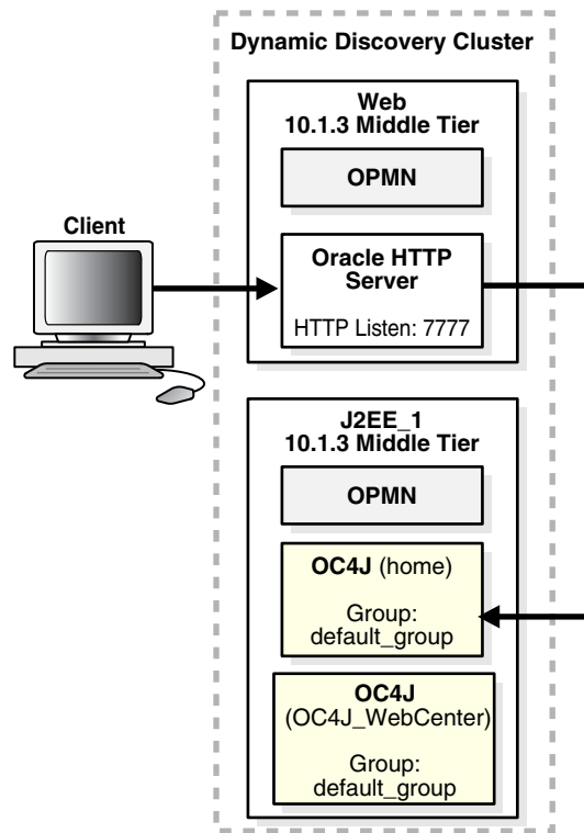
Figure 6–4 Web Server Middle Tier and Oracle WebCenter Framework Middle Tier on Separate Hosts in a Cluster
