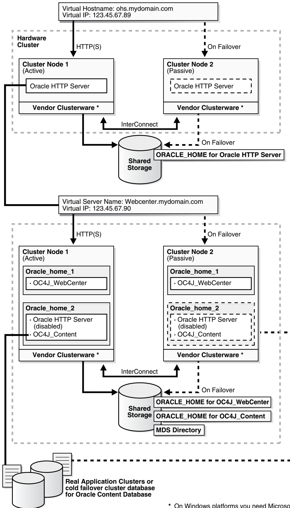
Figure 4-2 Active-Passive Topology with Components in Separate Oracle Homes
