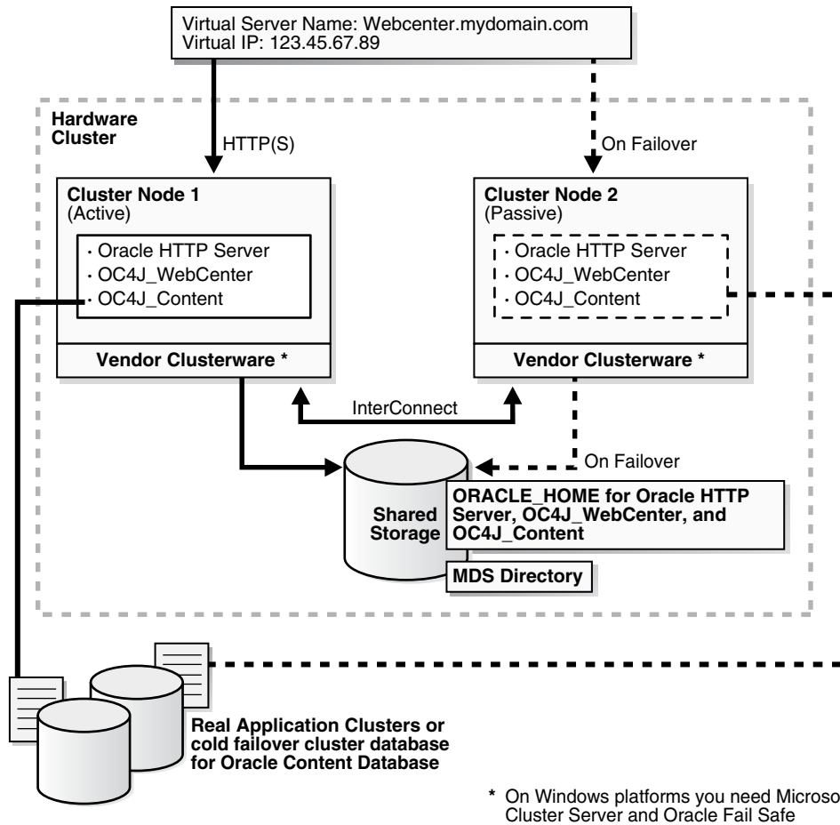
Figure 4–1 Active-Passive Topology with Oracle HTTP Server and WebCenter Suite in the Same Oracle Home
