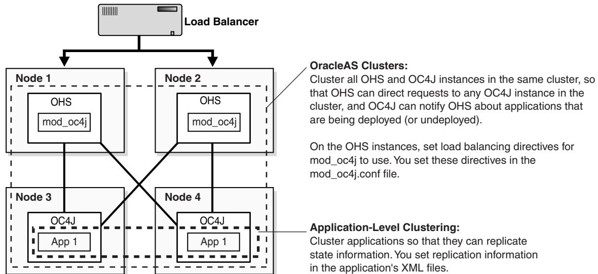
Figure 3–6 OracleAS Clusters and Load Balancing Directives
