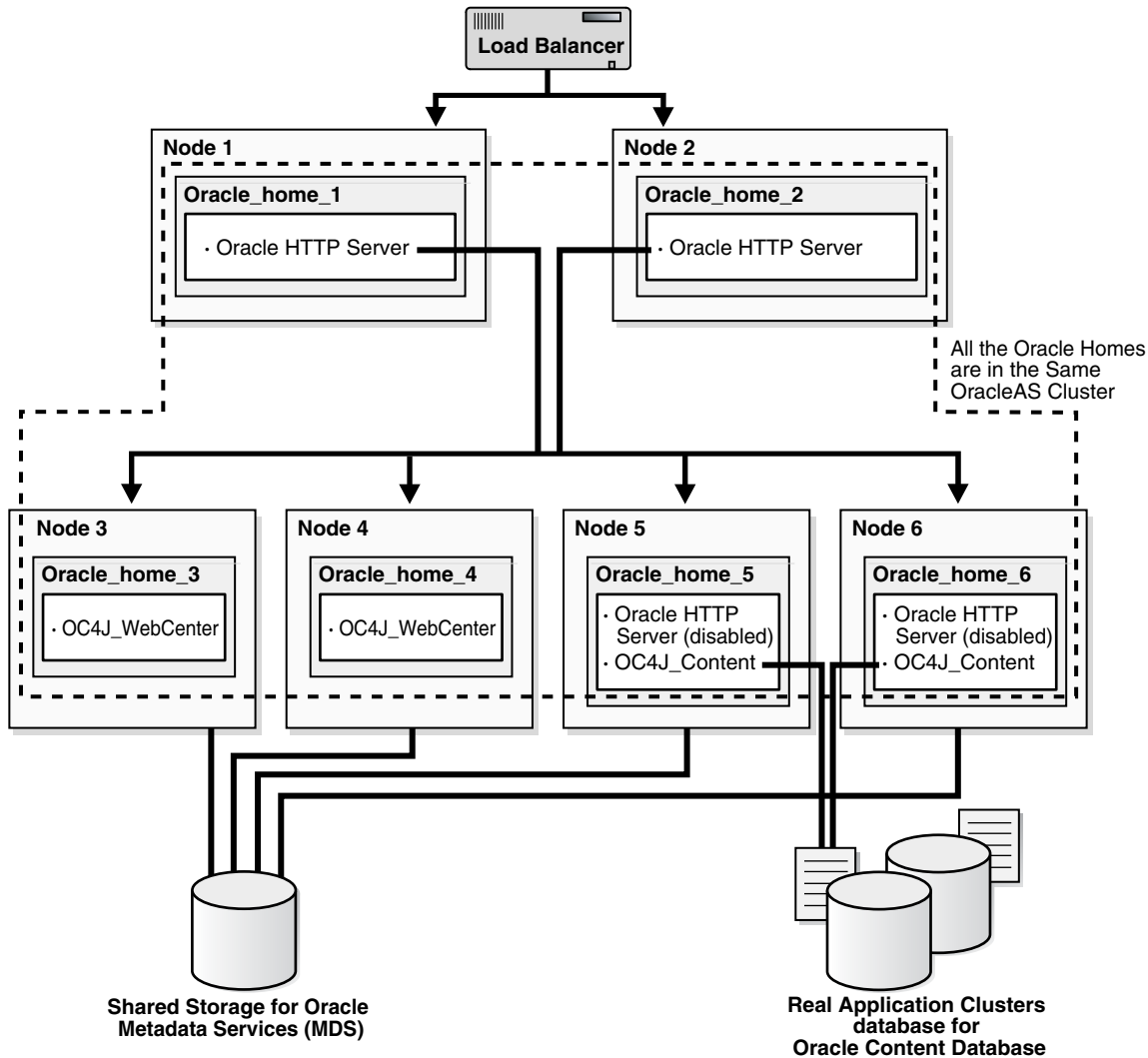
Figure 3–2 Active-Active Topology with Oracle HTTP Server, WebCenter Framework, and Oracle Content DB in Separate Oracle Homes
