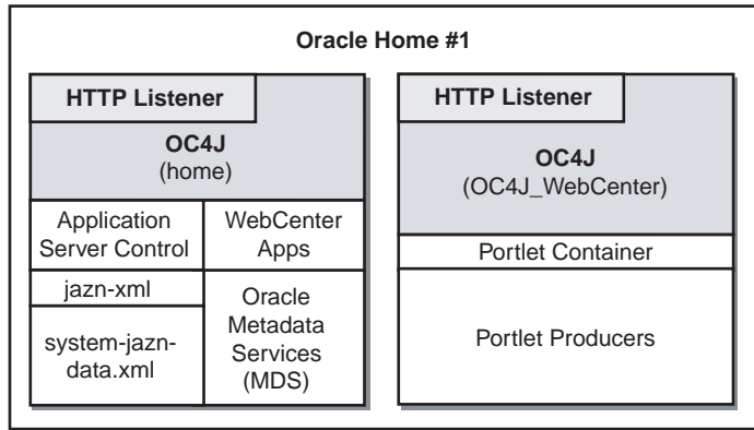
Figure 1–2 Oracle WebCenter Framework Only
