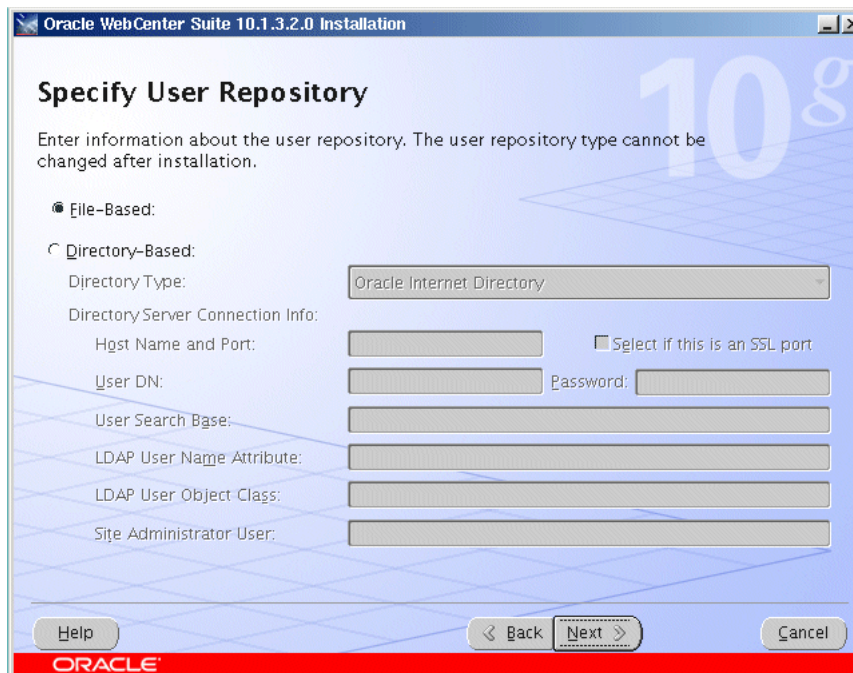
Figure 5–8 Oracle Universal Installer: Specify User Repository Screen
