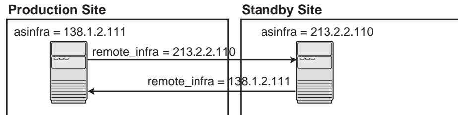
Figure 6–7 Entry for Oracle Data Guard in the Internal DNS Servers
