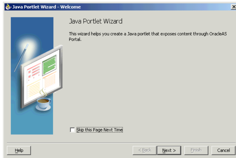
Figure 6–33 Welcome Page
