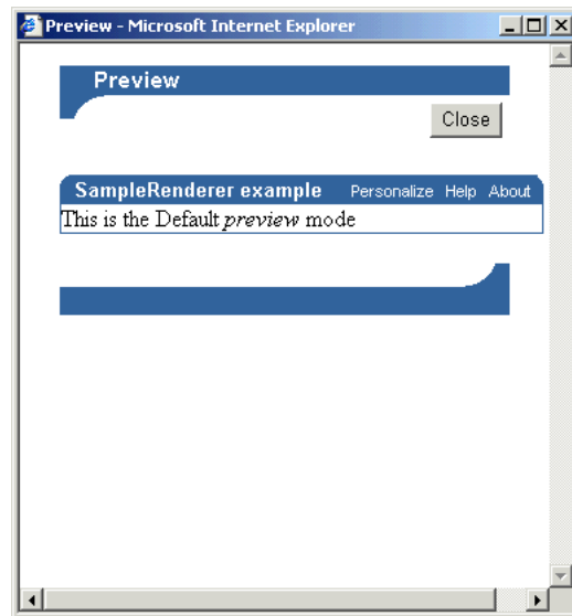
Figure 7-4 Preview Window
