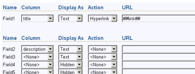
Figure 4-11 Column Layout Section of the Layout Tab
