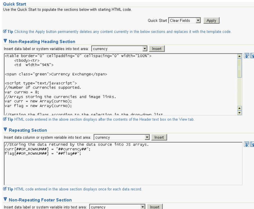
Figure 3–26 shows an example of an OmniPortlet using the HTML layout.
