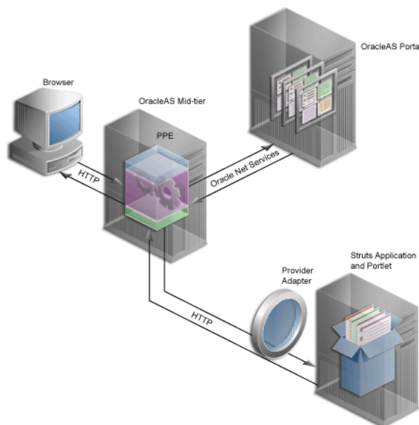
Figure 7–15 Integrating Struts Applications with OracleAS Portal
