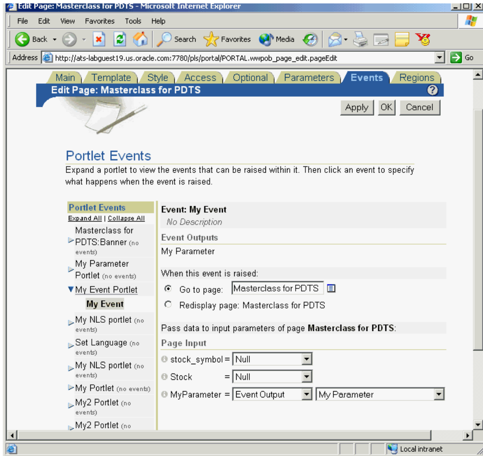
Figure 7-7 Portlet Events in the Edit Page
