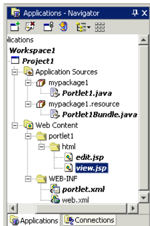
Figure 6–27 Application Navigator
