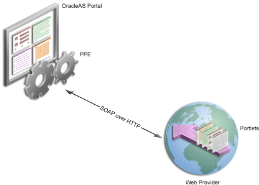
Figure 2–2 Web Providers
