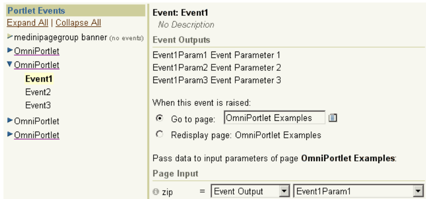
Figure 4–49 Page Input on the Events Tab
