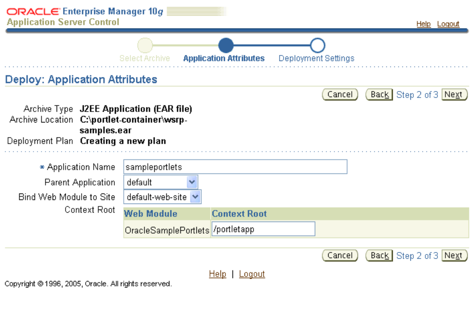
Figure 6–6 Deploy: Application Attributes Page
