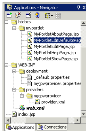
Figure 6–41 Application Navigator
