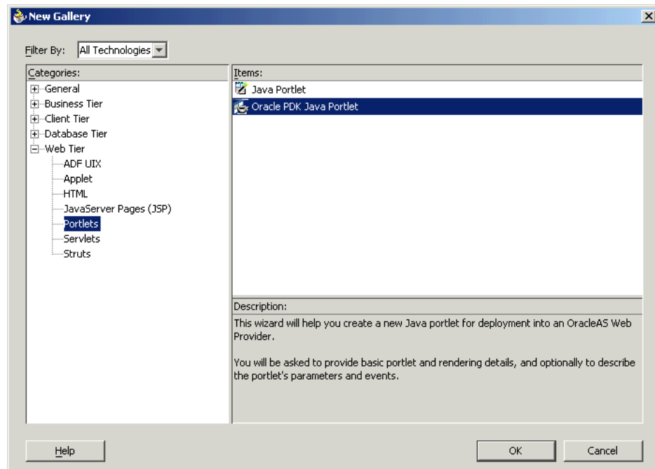
Figure 6–32 New Gallery Dialog Box for Oracle PDK Java Portlet
