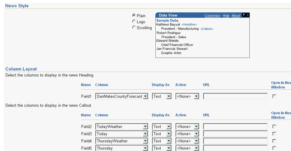
Figure 4–33 Layout Tab
