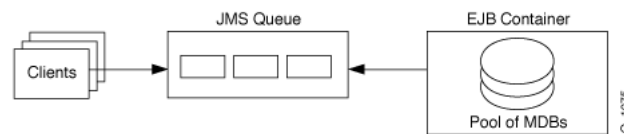
Figure 1-7 Message Driven Beans
