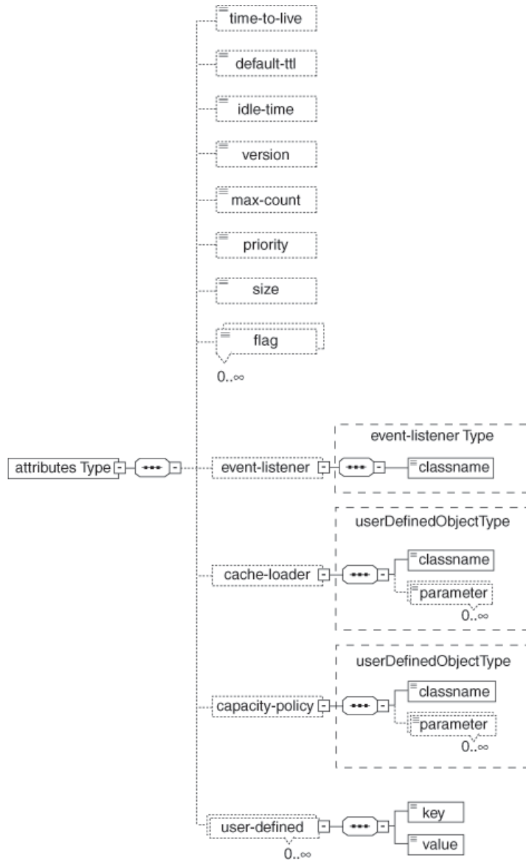
Figure 7-6 Declarative Cache Schema Attributes
