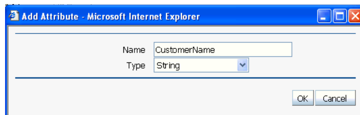
Figure 5–80 Add Attribute
