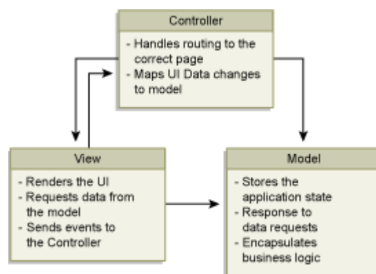
Figure 19–7 MVC Pattern
