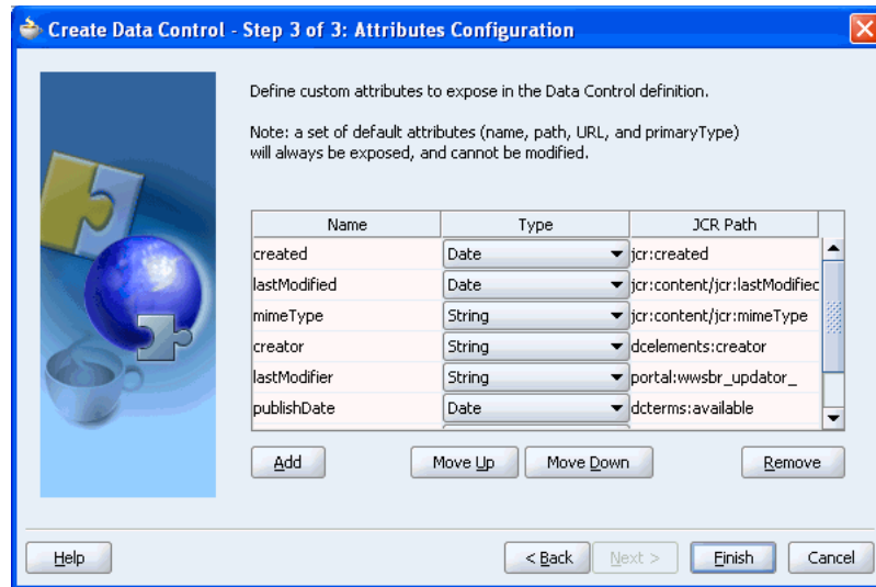
Figure 5–8 Attributes Configuration
