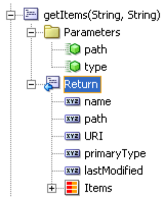
Figure 5–42 SRFileSystem.getItems
