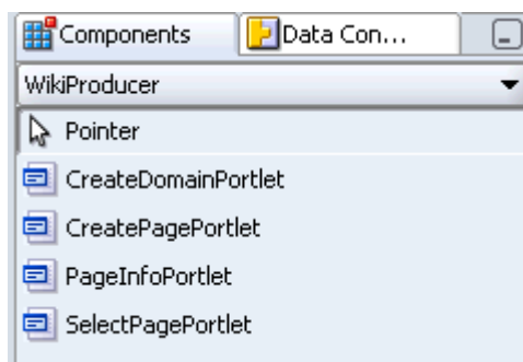
Figure 6-17 Component Palette
