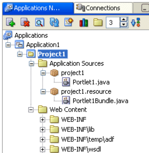
Figure 18–19 Example of Files Generated for a JPS-Compliant Portlet
