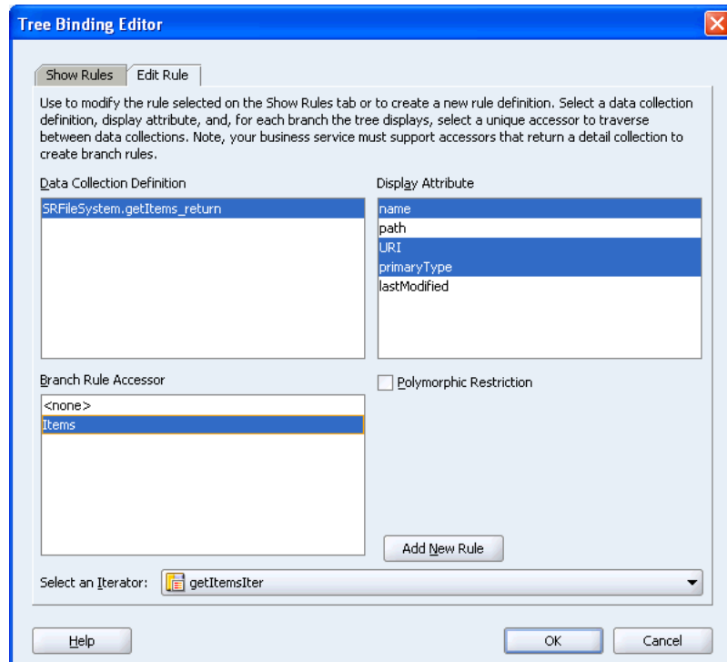
Figure 5–57 Tree Binding Editor
