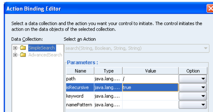
Figure 5–62 Action Binding Editor - search
