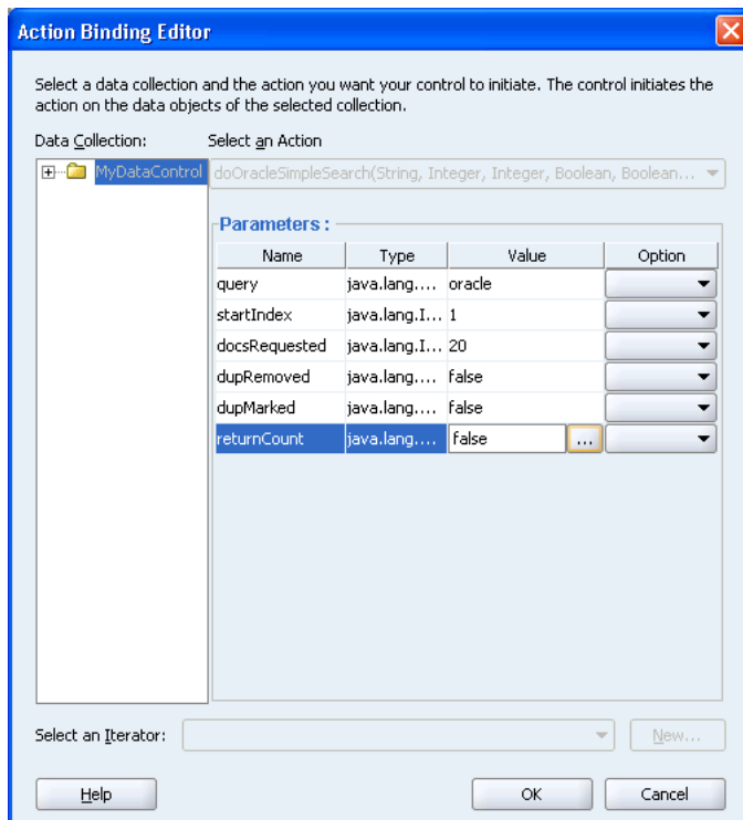
Figure 8–4 Action Binding Editor
