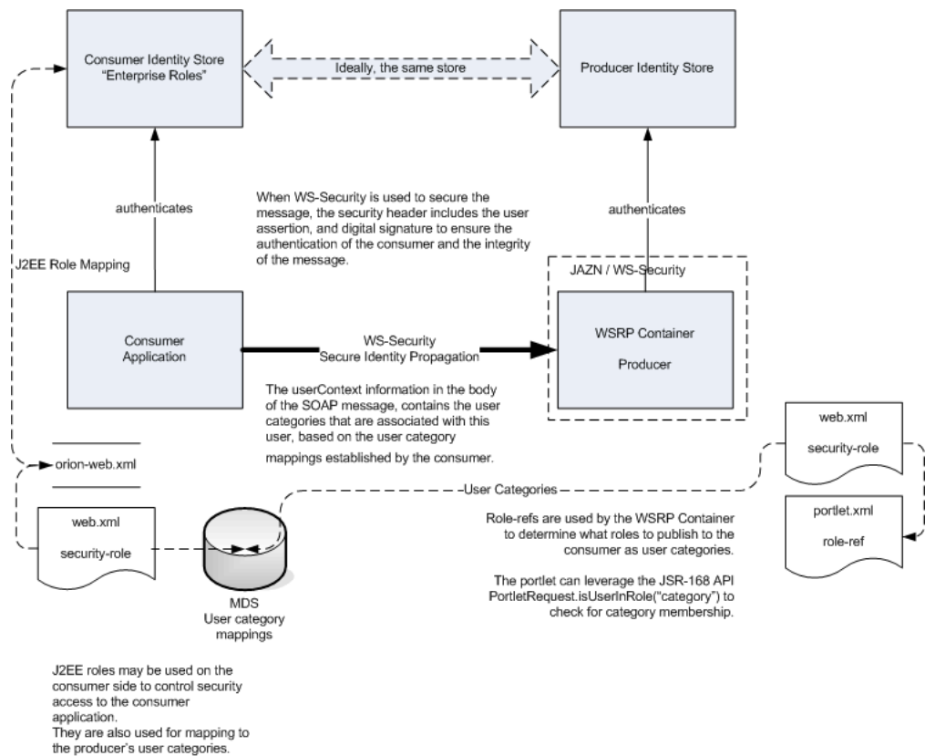
Figure 10-47 WSRP Portlet Security Architecture
