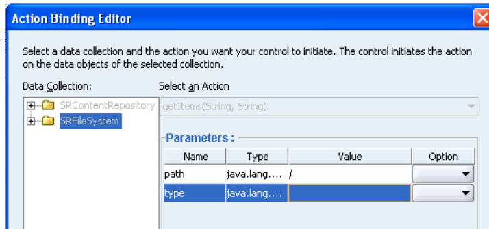
Figure 5–44 Action Binding Editor
