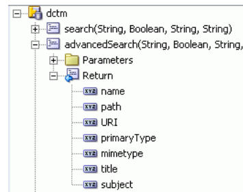
Figure 5–74 Custom Attributes under
