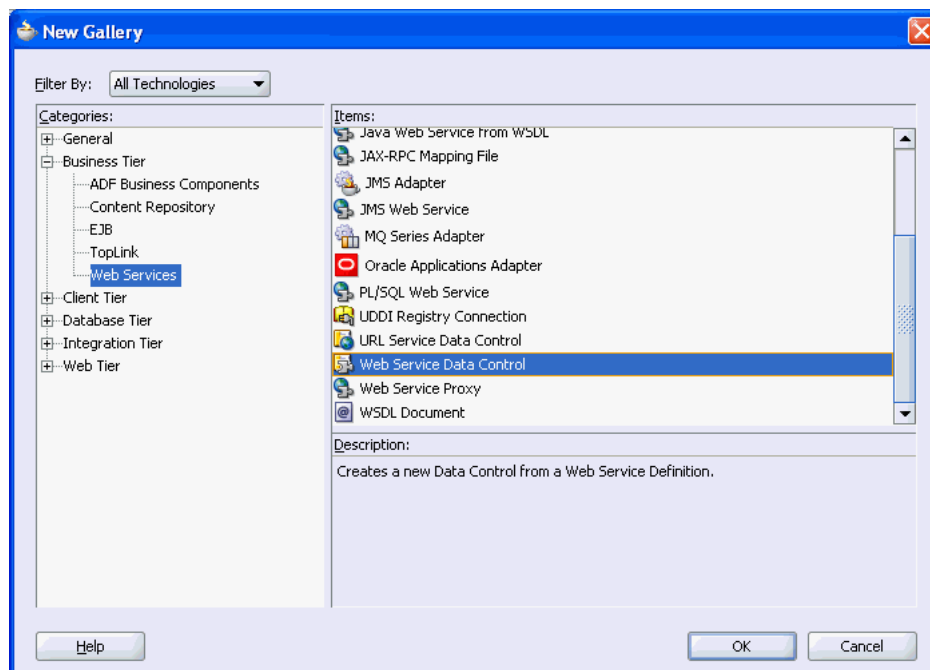
Figure 5–88 New Gallery - Web Service Data Control
