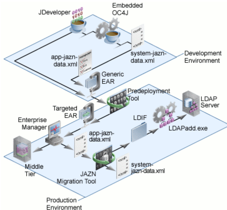
Figure 12–4 Deployment of a WebCenter Application to an OC4J in Oracle Application Server
