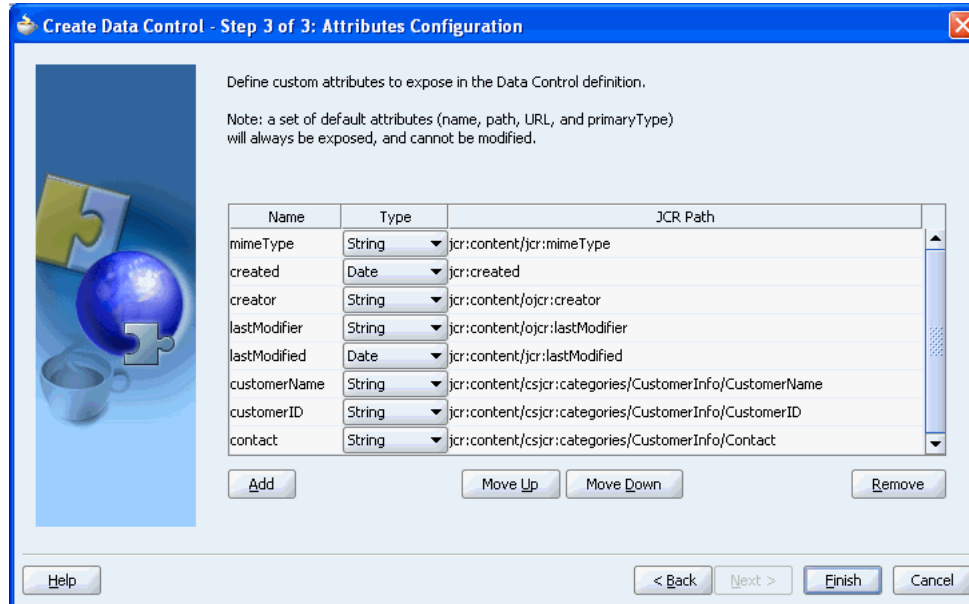
Figure 5–86 Attributes Configuration Page
