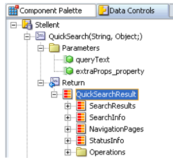
Figure 5–107 The Return Node - QuickSearchResult
