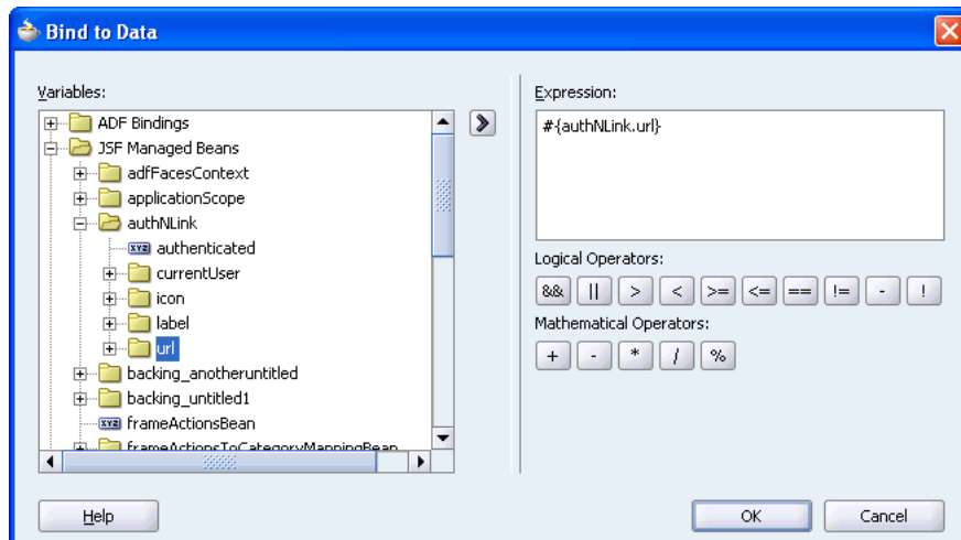
Figure 10–30 Bind to Data Dialog Box for the Destination Property
