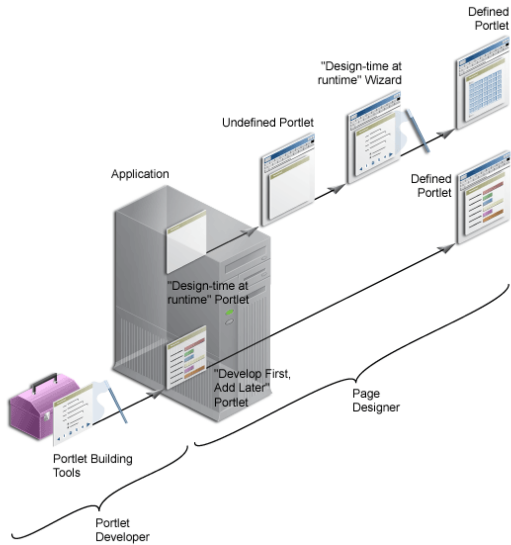
Figure 15-4 Portlet Creation Style
