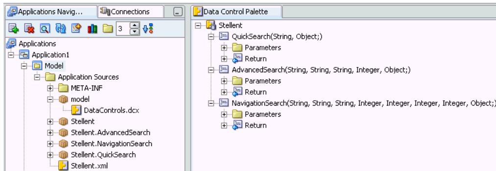
Figure 5–92 Stellent Data Control in the Applications Navigator and the Data Control Palette
