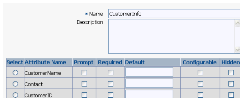
Figure 5–81 Attributes of the CustomerInfo Category
