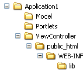
Figure 3–2 Application from WebCenter Application Template in a Windows File System
