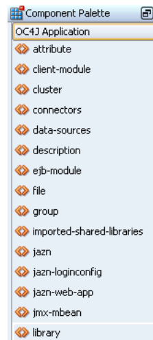
Figure 12–12 Library Option
