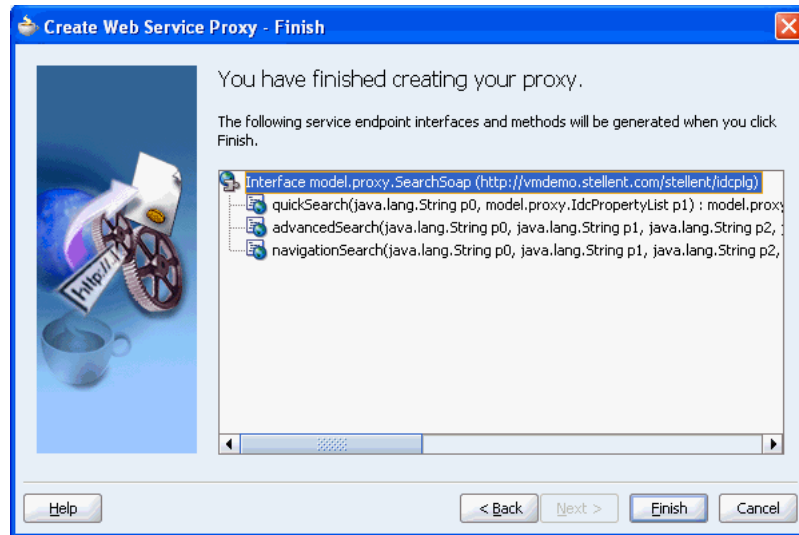
Figure 5–100 Finish Page
