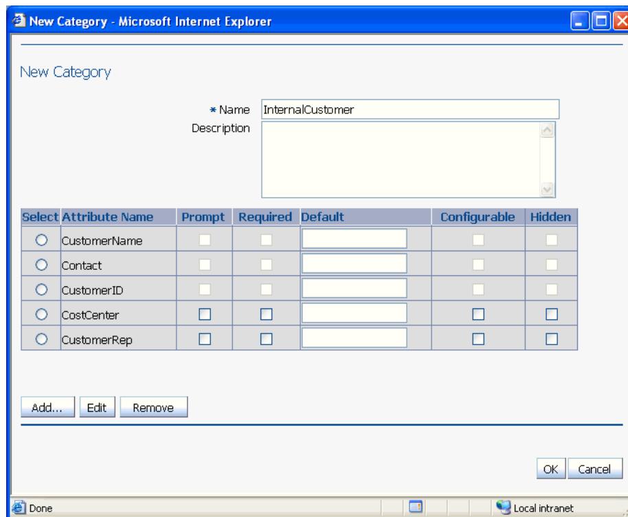
Figure 5-83 New Category
