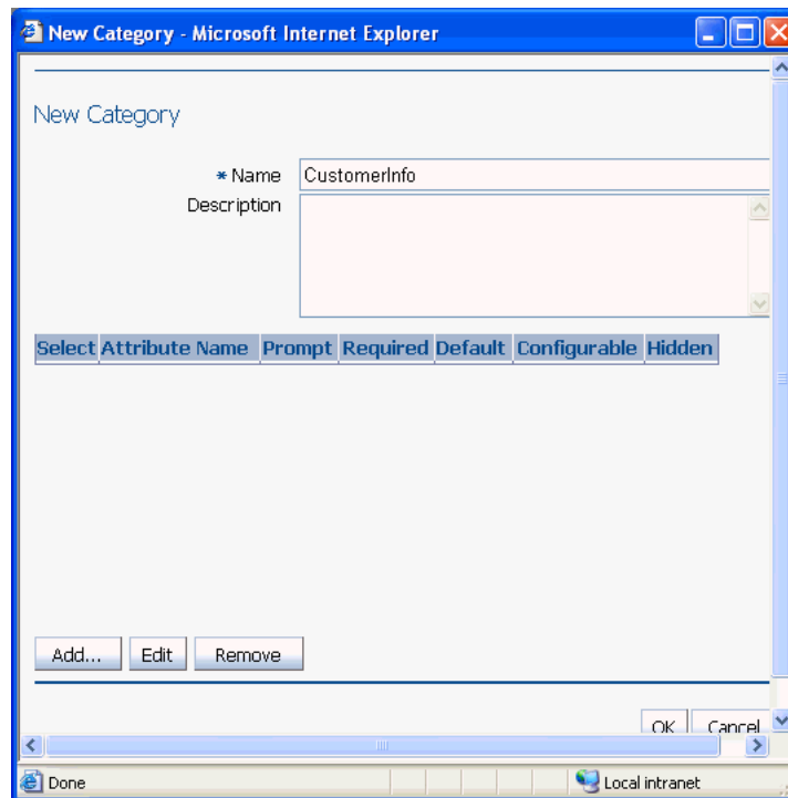
Figure 5–79 New Category
