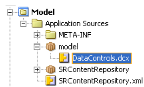
Figure 5–22 DataControls.dcx
