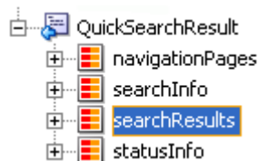
Figure 5–112 searchResults
