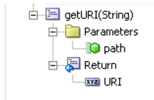
Figure 5–28 SRFileSystem.getURI
