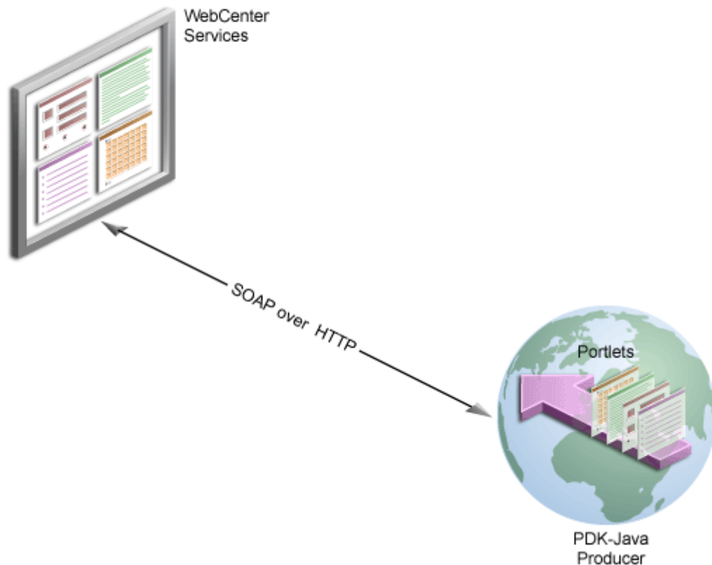
Figure 15–2 PDK-Java Producers
