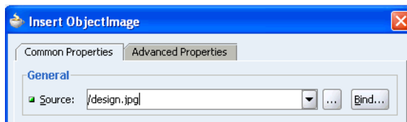
Figure 5-36 Insert ObjectImage
