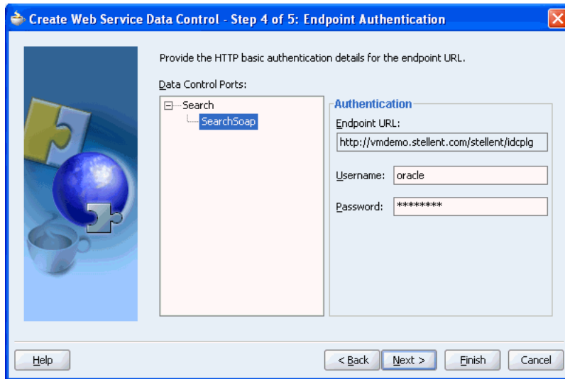
Figure 5–91 Endpoint Authentication
