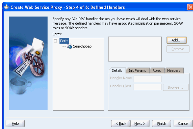
Figure 5–97 Defined Handlers
