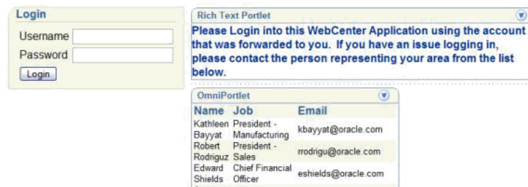
Figure 10–33 Login Page
