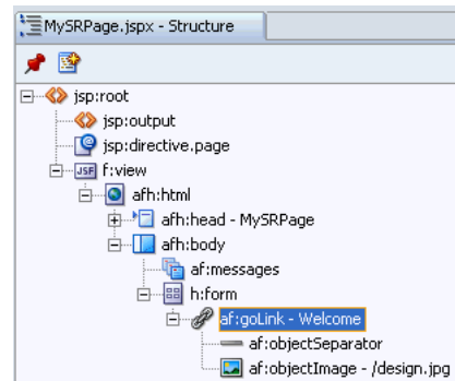
Figure 5–37 Structure Window
