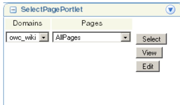
Figure 6–20 SelectPagePortlet
