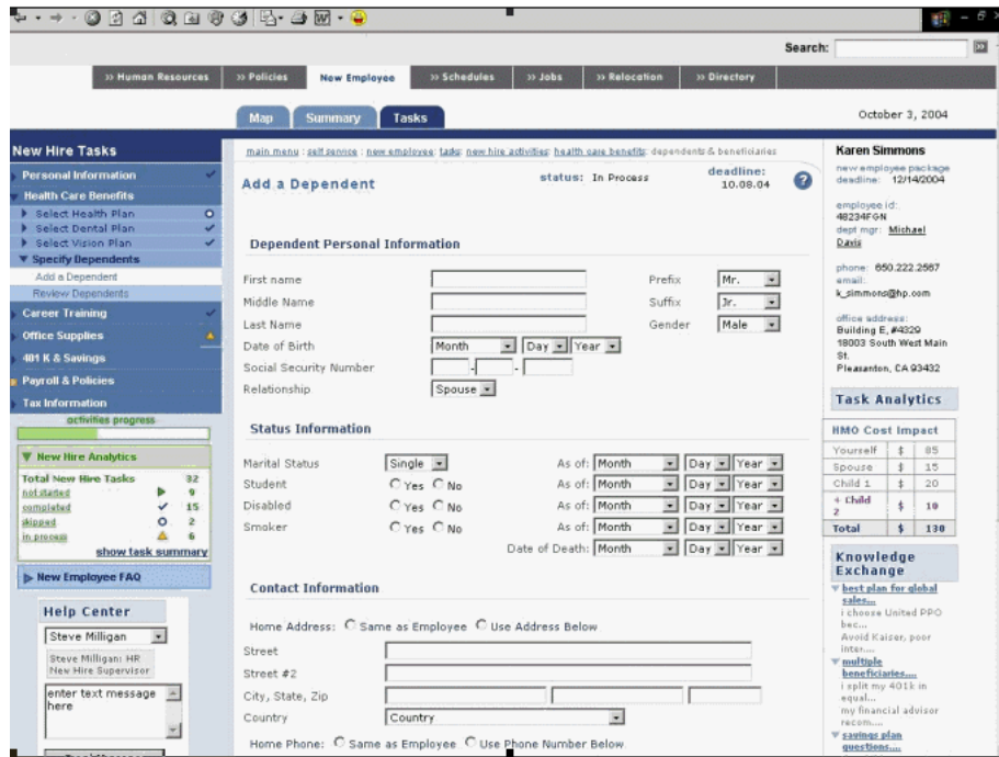
Figure 1-1 Sample Application
