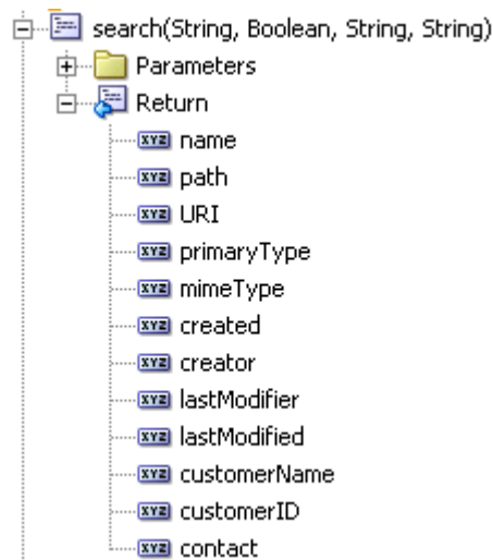
Figure 5–87 Custom Attributes
