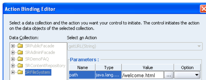
Figure 5–30 Action Binding Editor
