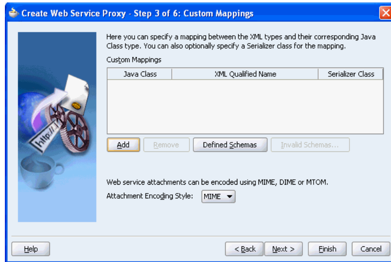
Figure 5–96 Custom Mappings
