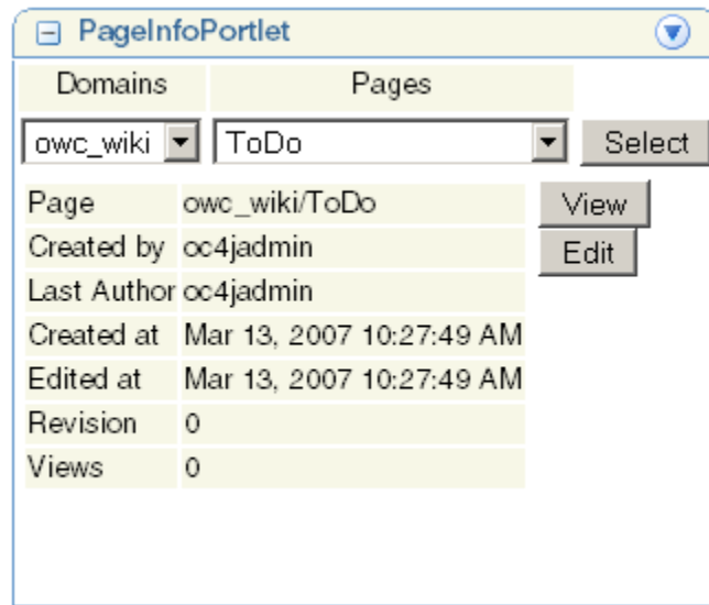
Figure 6–22 PageInformation Portlet
