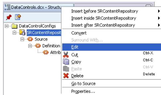
Figure 5–24 Context Menu
