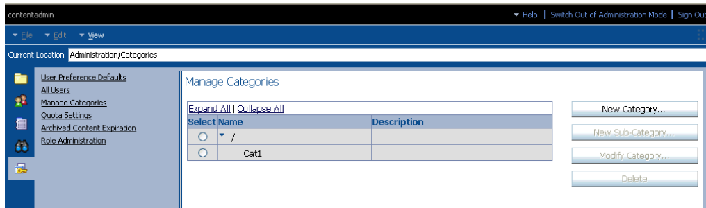
Figure 5–78 Manage Categories
