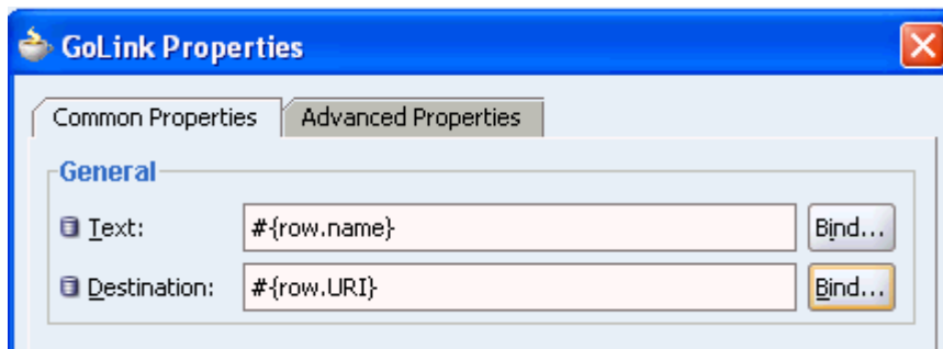
Figure 5–49 GoLink Properties
