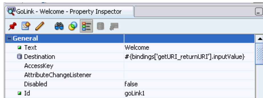
Figure 5-31 GoLink Properties
