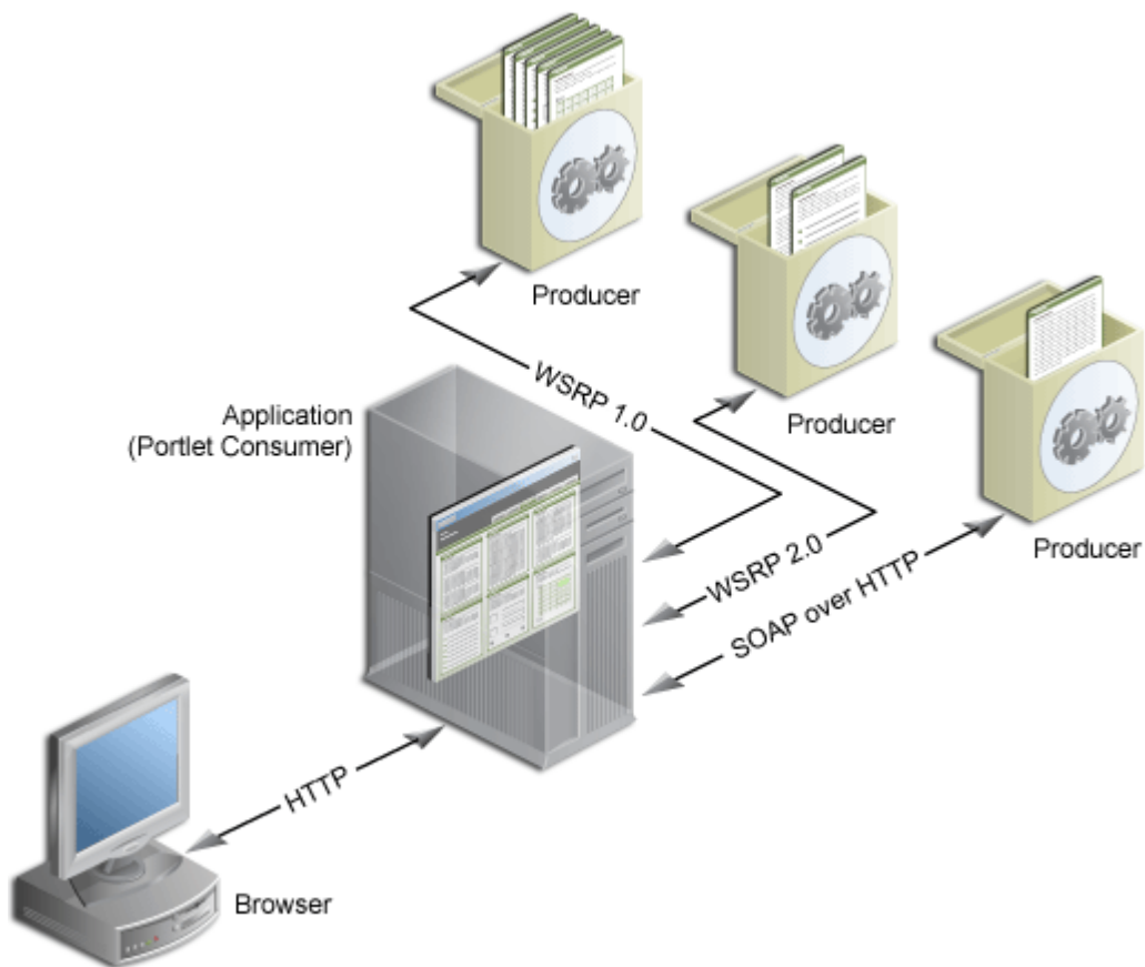
Figure 15–3 Producer Architecture
