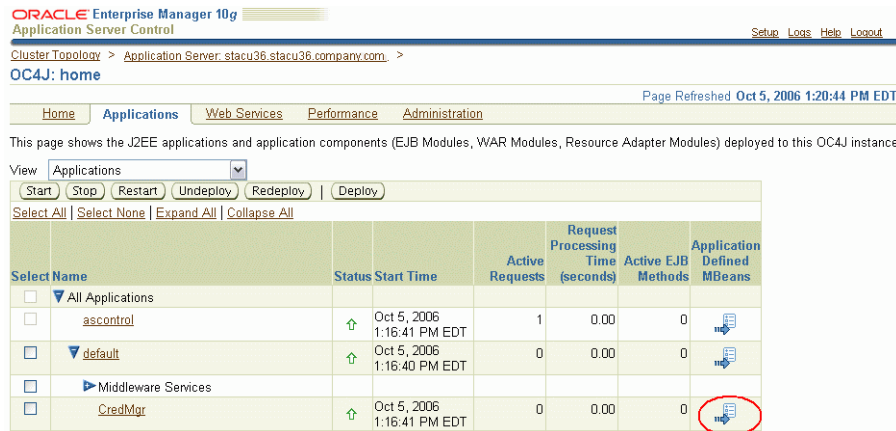
Figure 12–26 Applications Tab
