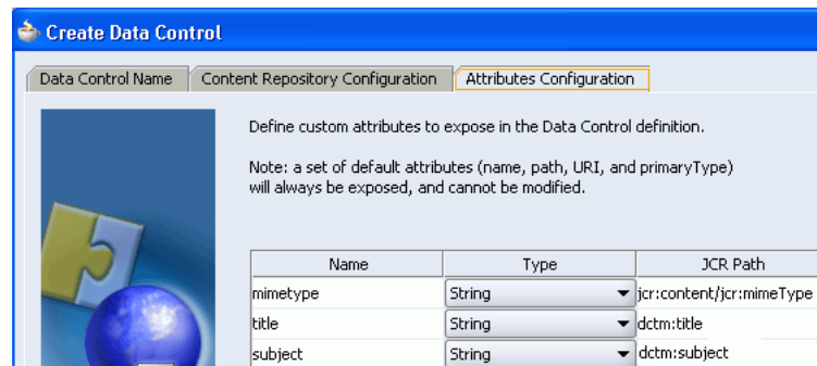
Figure 5–73 Custom Attributes
