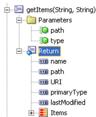
Figure 5–54 SRFileSystem.getItems
