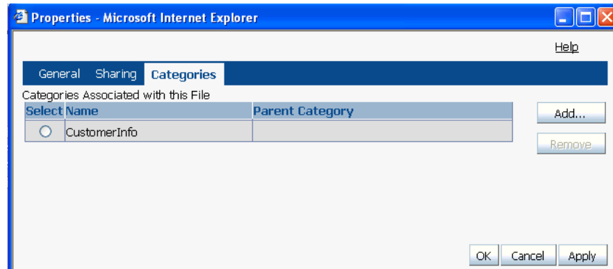
Figure 5–84 Properties Window
