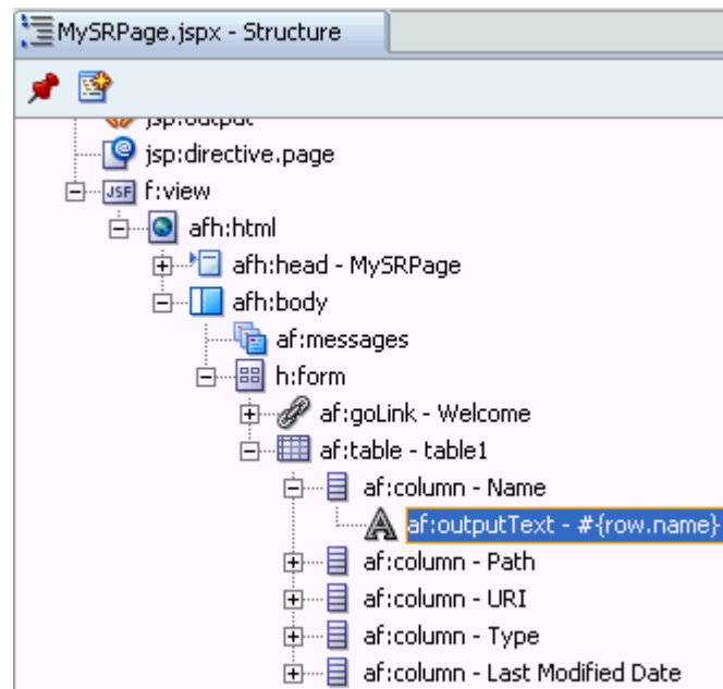
Figure 5-47 Default Formatting for the Name Column
