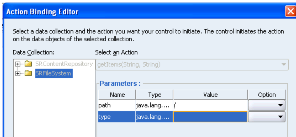
Figure 5–56 Action Binding Editor
