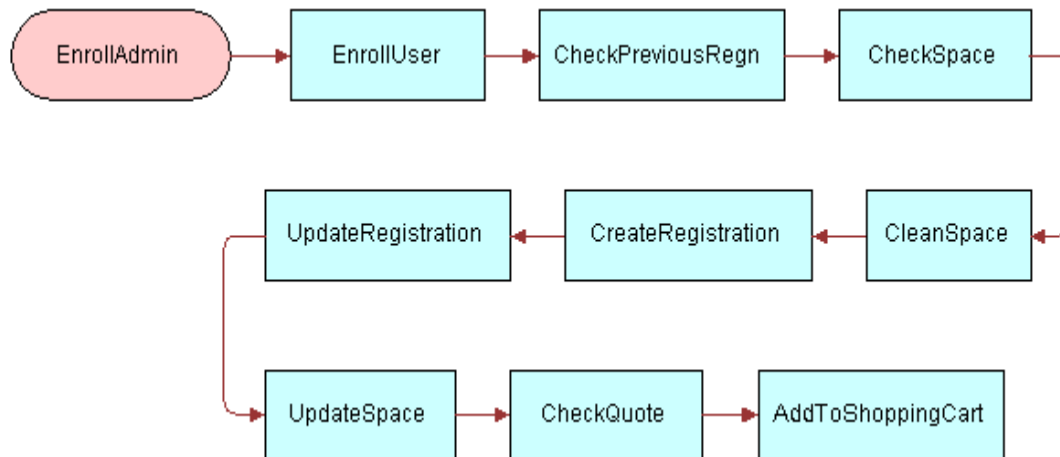
Figure 11. EventRegistrationService Flow
