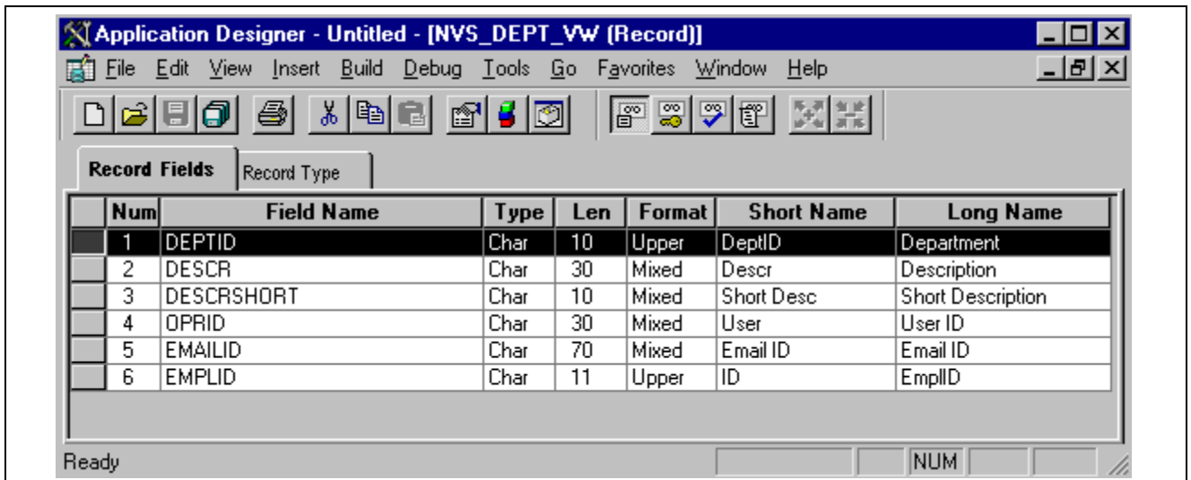
Application Designer: NVS_DEPT_VIEW page
