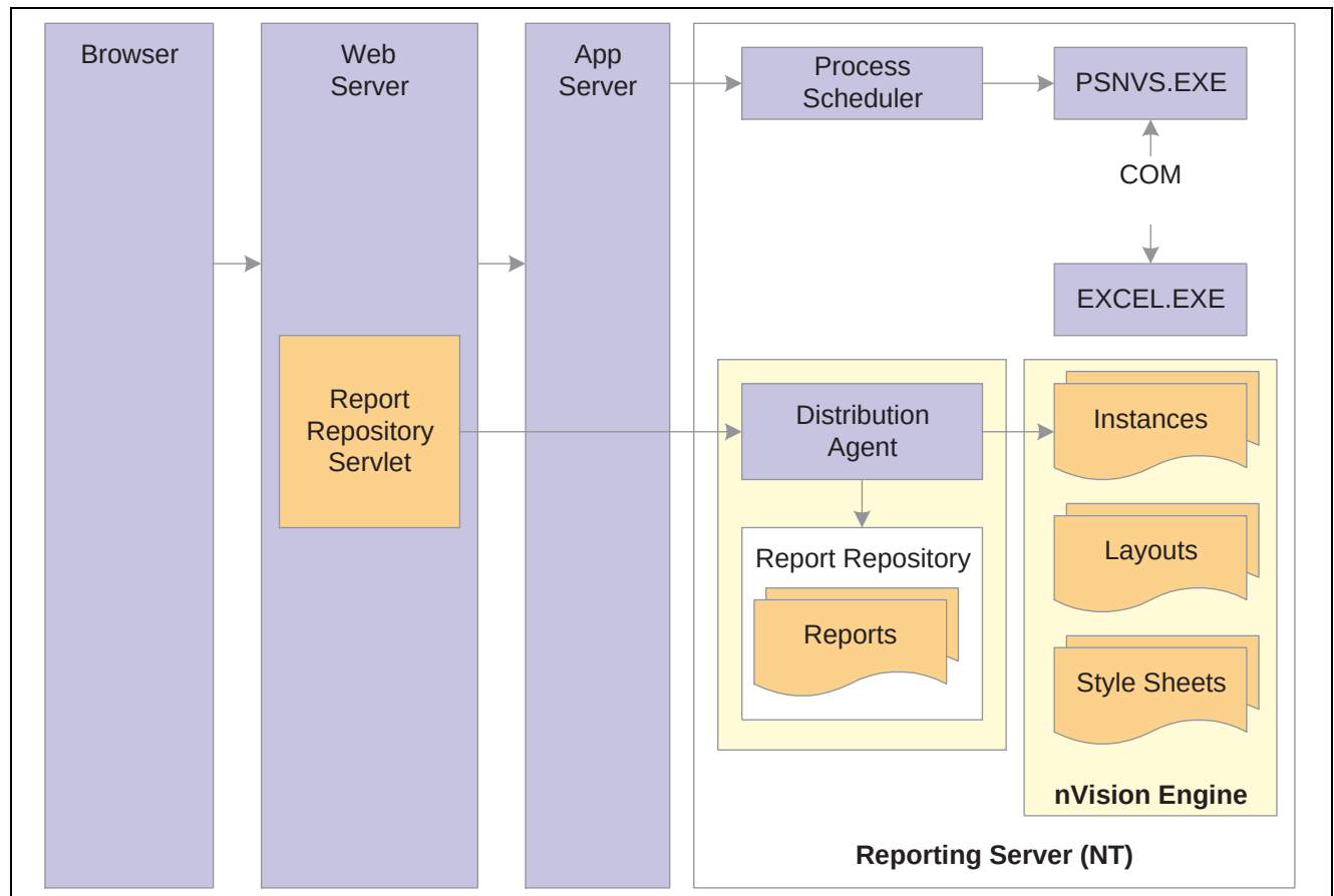
nVision Architecture – Web version
