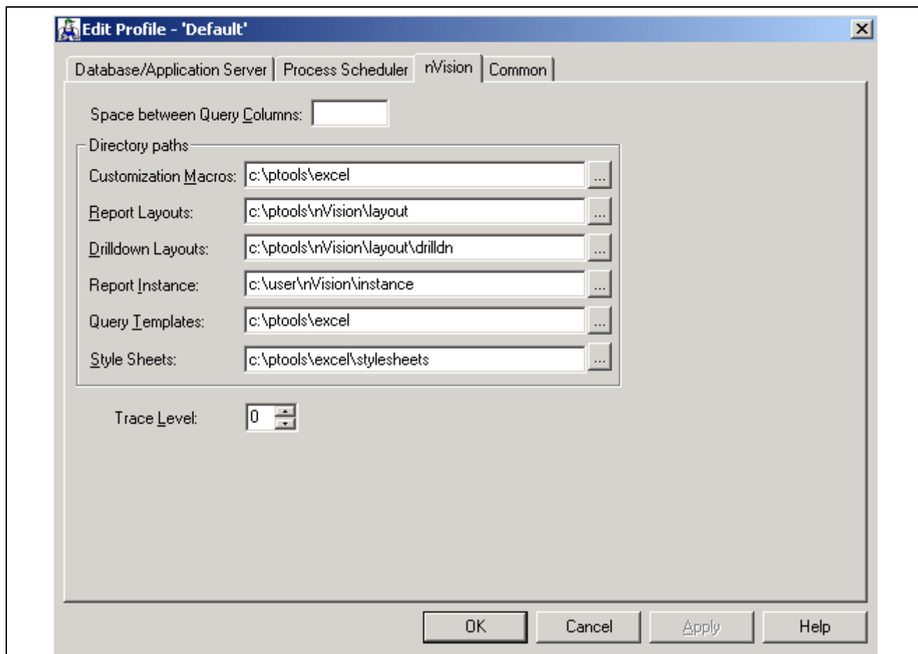
Configuration Manager – General settings for nVision
