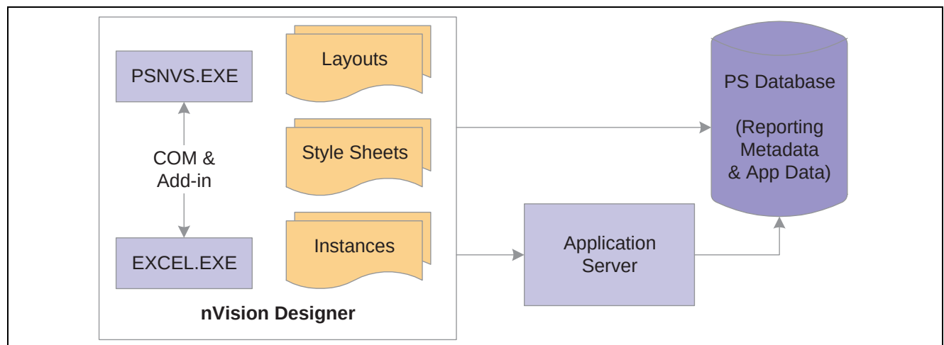
nVision Architecture – Windows version
