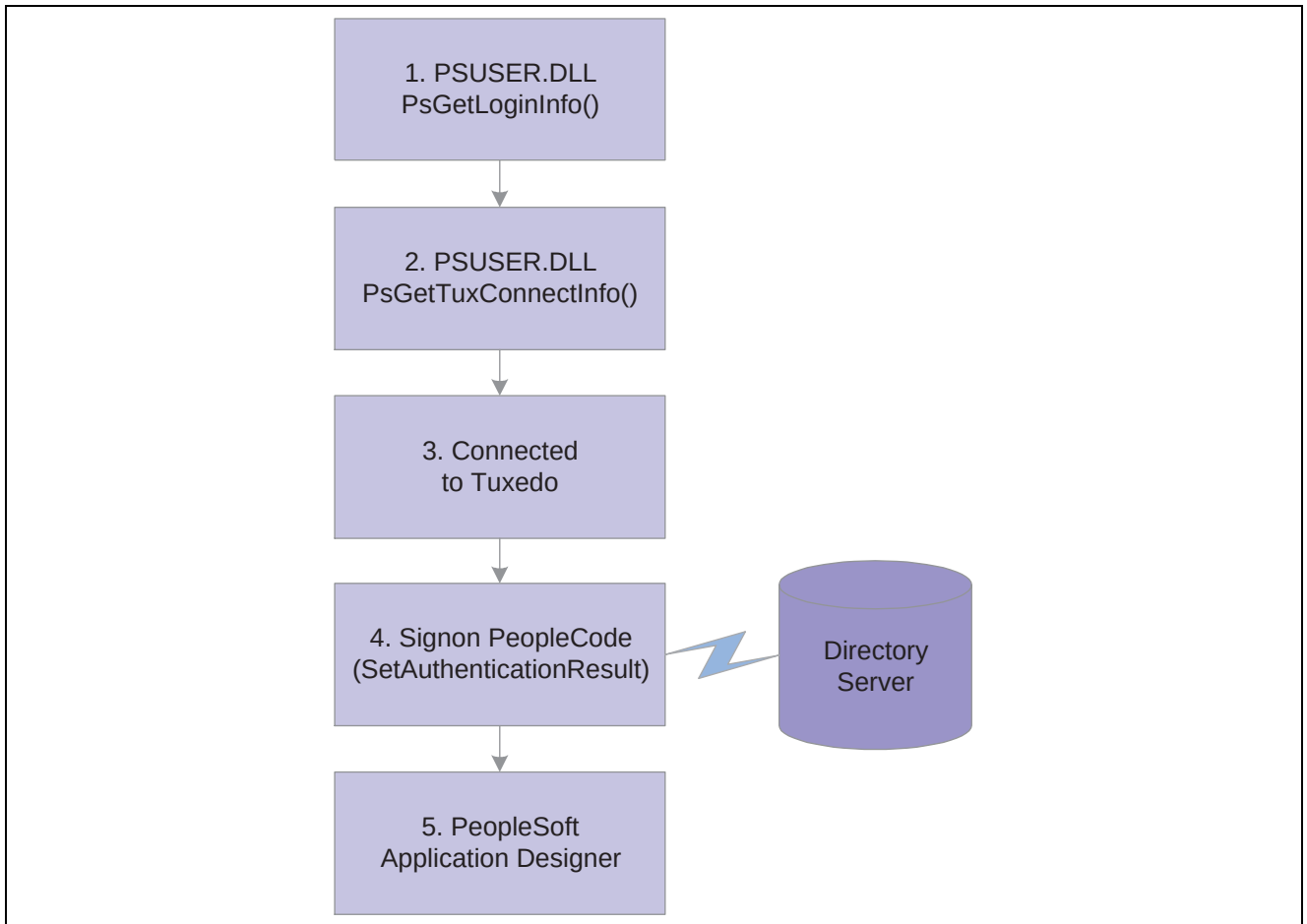
Microsoft Windows Client three-tier signon exits
