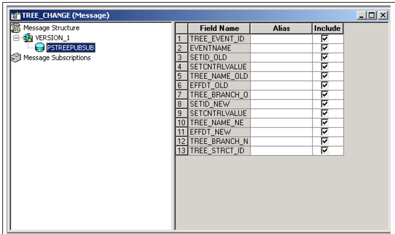
Application Designer - Tree Change (service operation)
