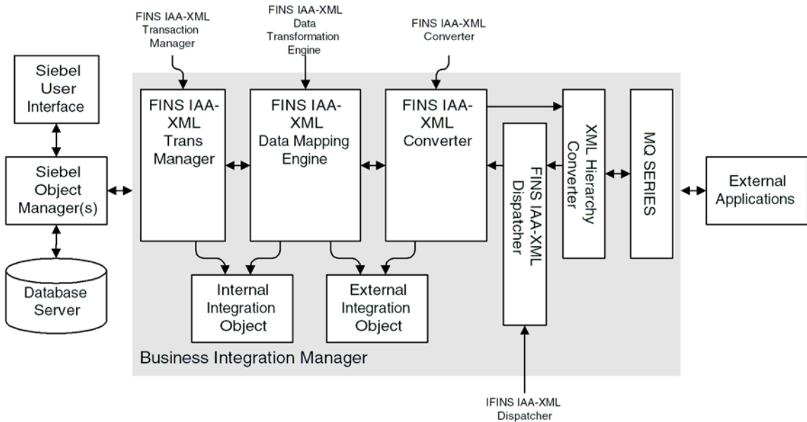
Figure 2. Bi-directional Business Data Flow of Siebel Connector for IAA-XML
