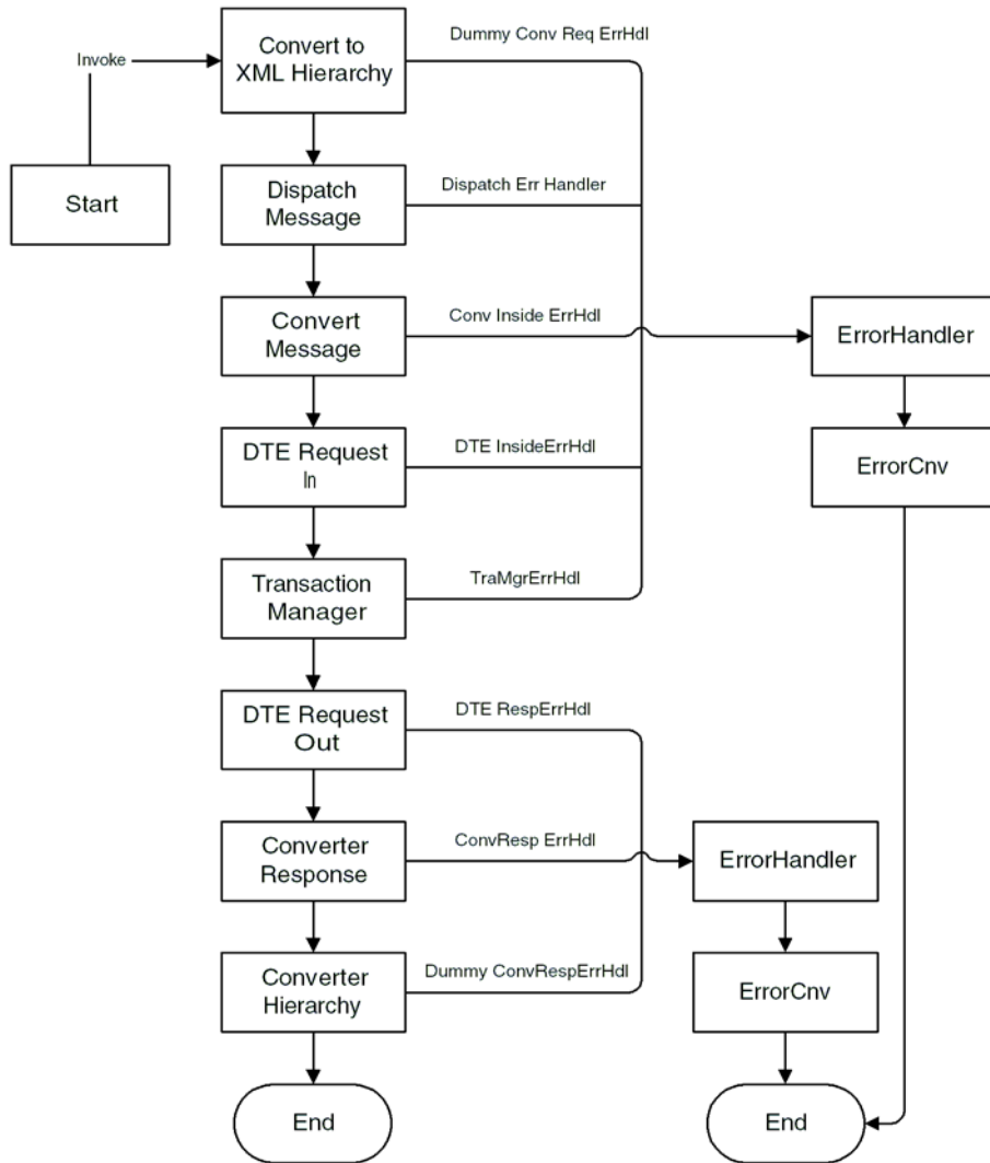
Figure 6. IAA Server Party Package Workflow
