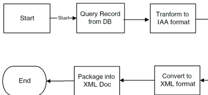
Figure 5. IAA Add Party Outbound Workflow
