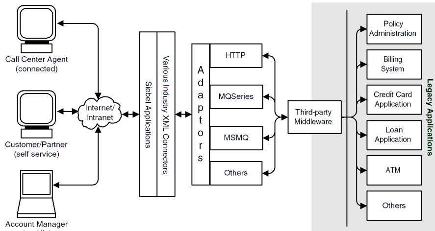
Figure 1. Legacy Encapsulation
