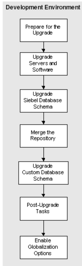
Figure 2. Upgrade of the Development Environment
