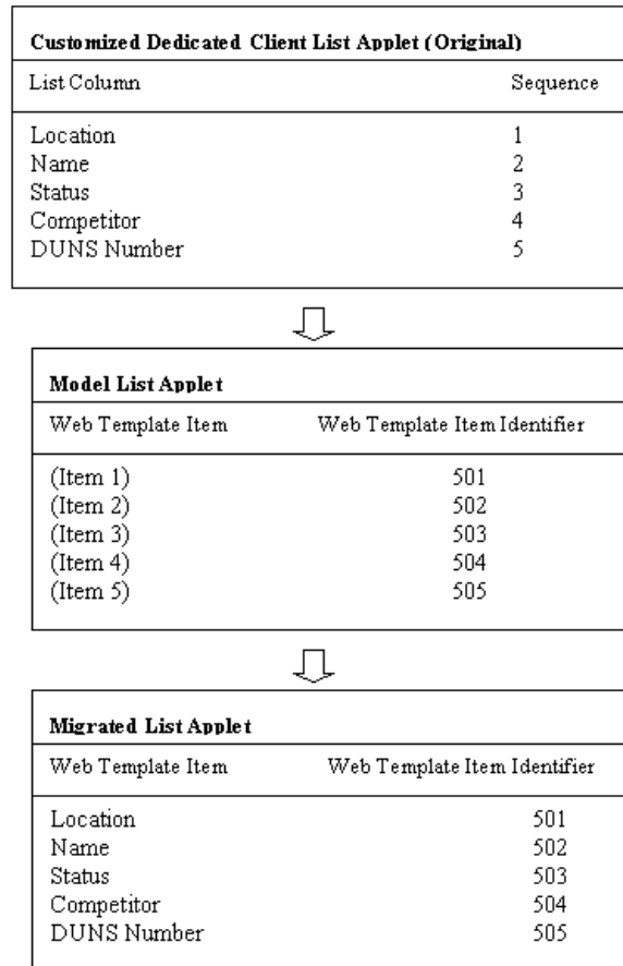
Figure 14. Migration of a Dedicated Client List Applet to a Web Client List Applet
