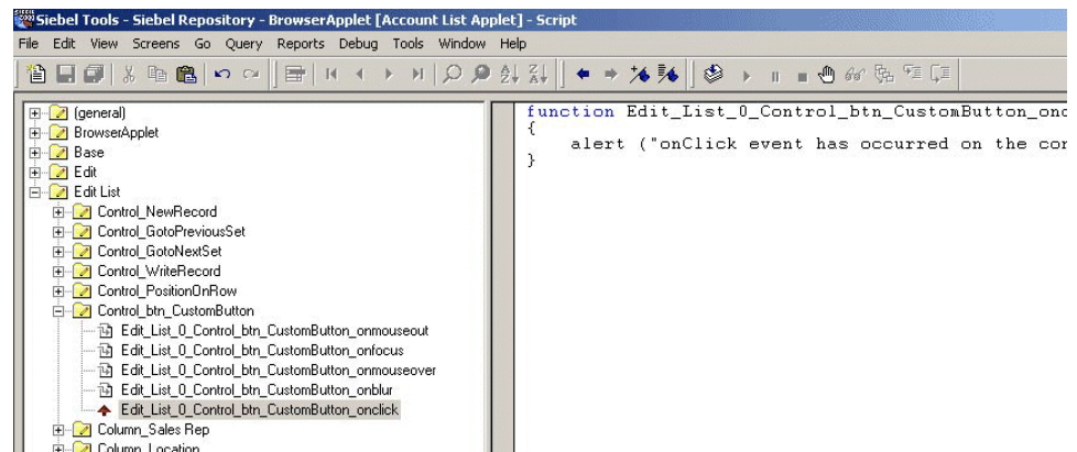
Figure 15. DOM Events When MiniButton Control Added to Applet
