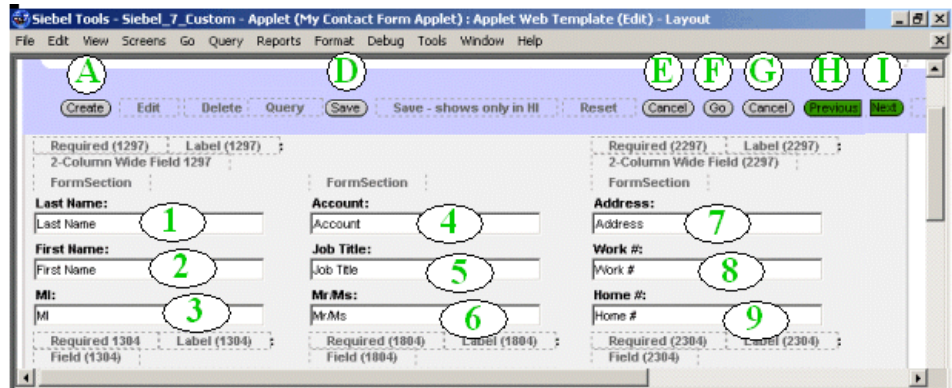
Figure 13. Migrated Acme Contact Form Applet
