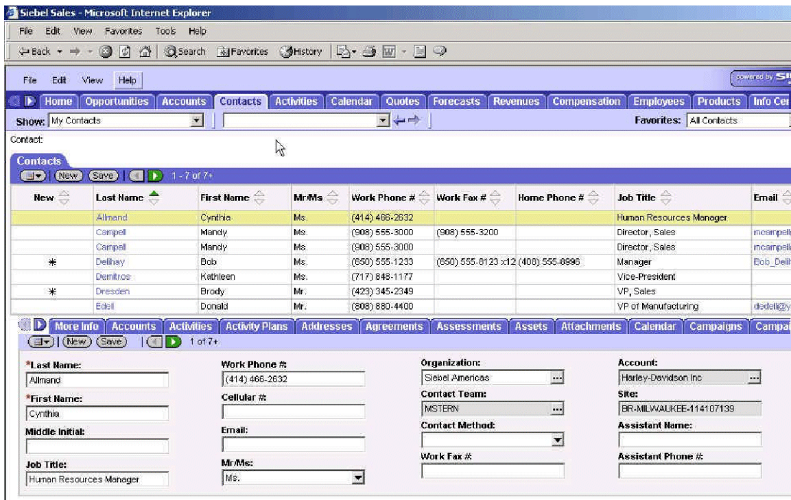
Figure 10. Contact List View – Web Client
