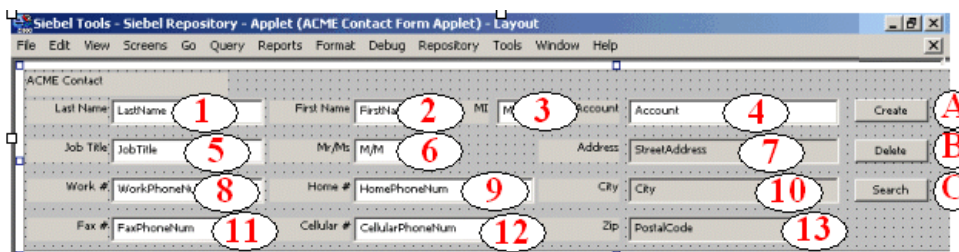
Figure 11. ACME Contact Form Applet in Siebel 2000 Applet Designer
