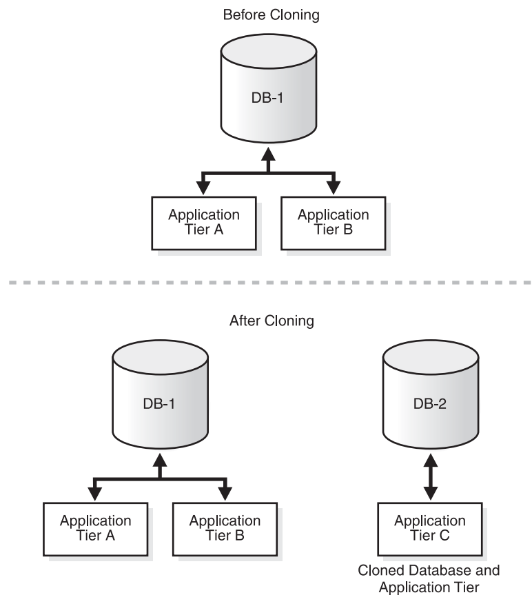
Figure 24–2 Site Cloning
