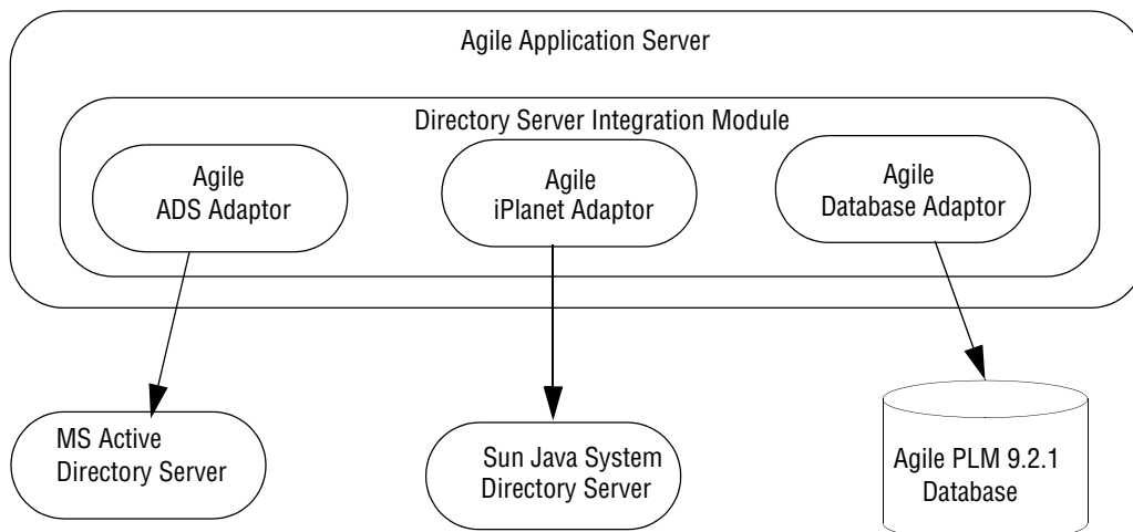
Figure 5-1: LDAP Architecture
