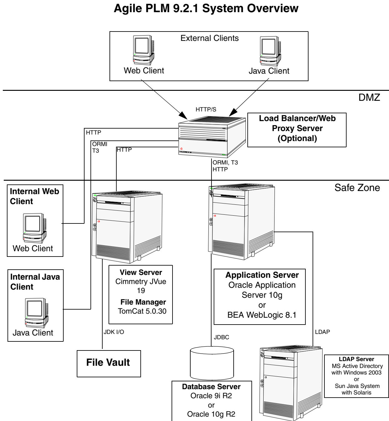
Figure 1-1: System Configuration Overview
