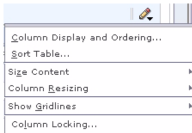
Figure 6–2 Drop-down Menu
