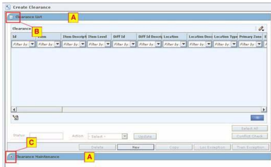
Figure 2–6 RPM Pane
