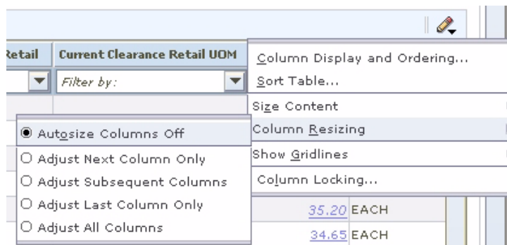
Figure 6–6 Column Resizing
