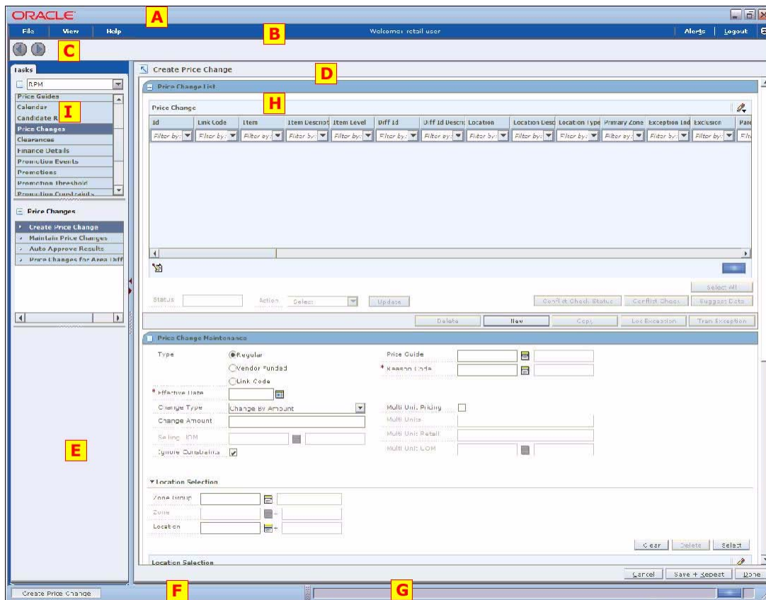
Figure 2–1 RPM Workspace
