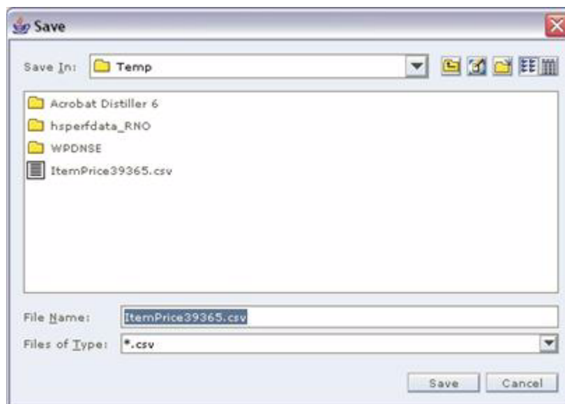
Figure 4–5 Save Window
