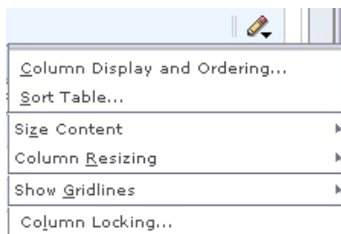
Figure 5–2 Drop-down Menu
