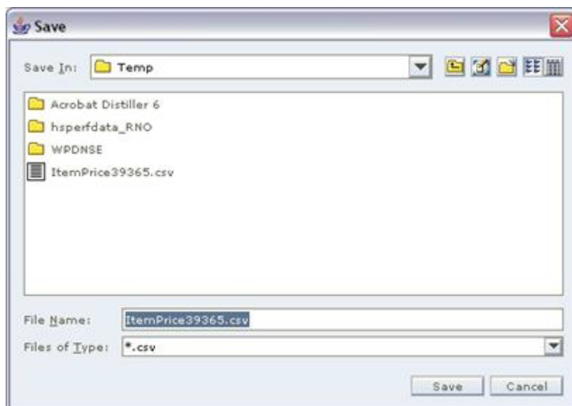
Figure 3–5 Save Window
