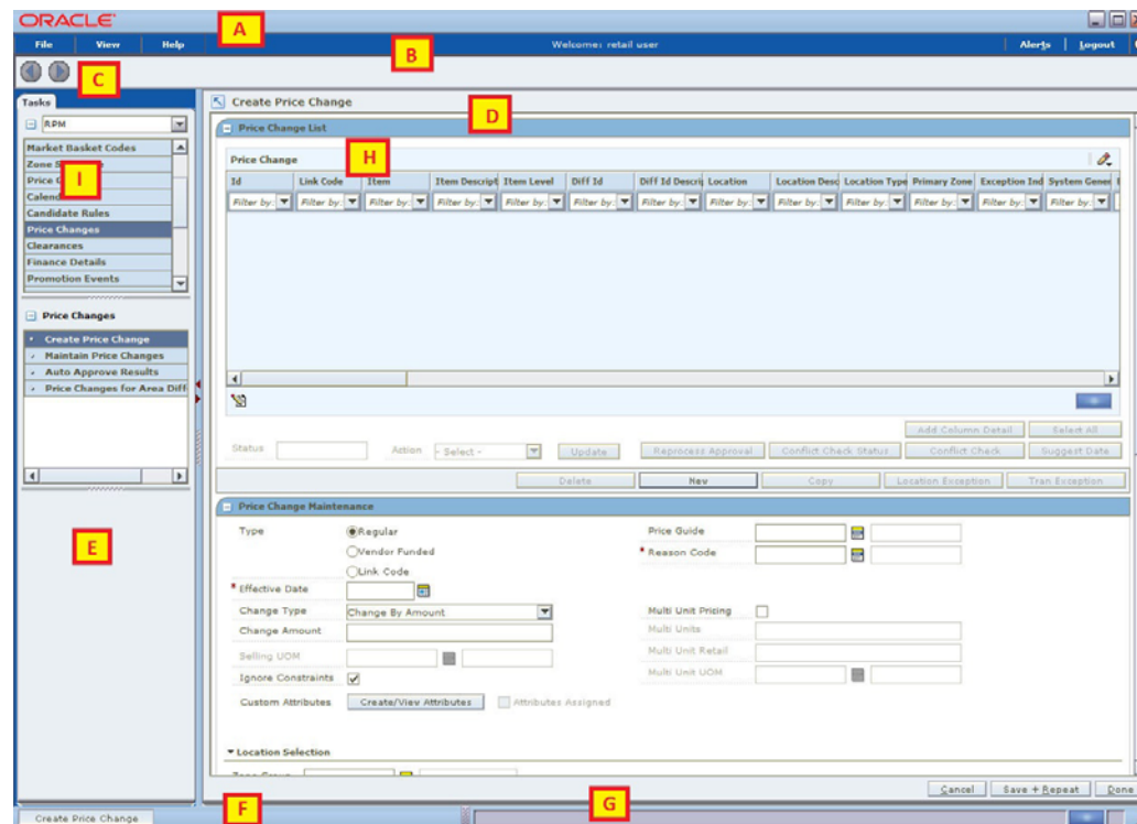
Figure 1–1 RPM Workspace
