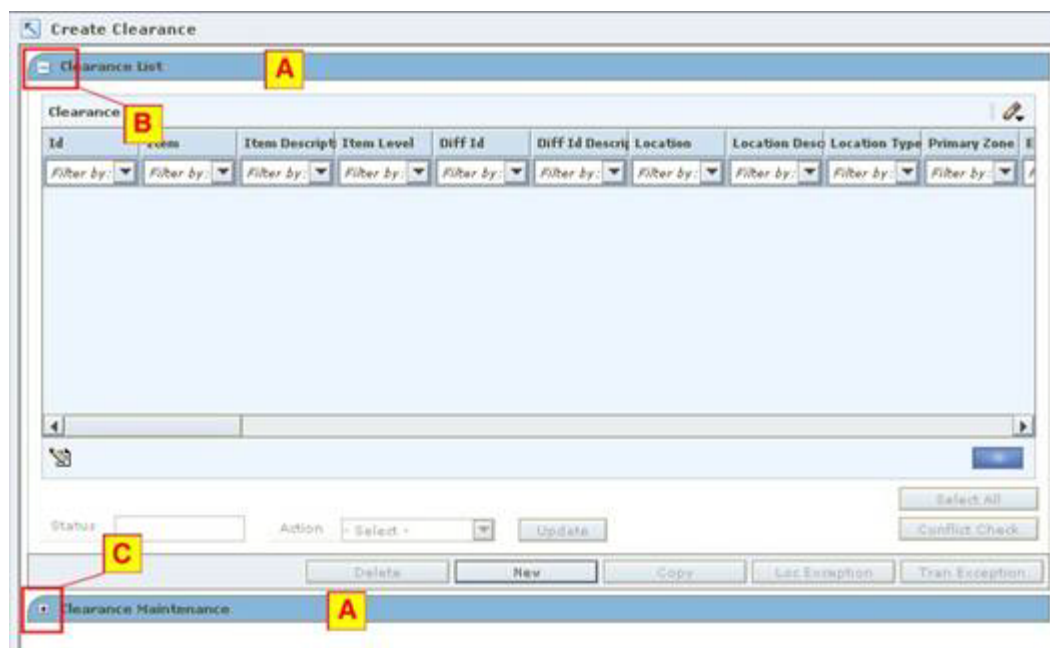
Figure 1–6 RPM Pane
