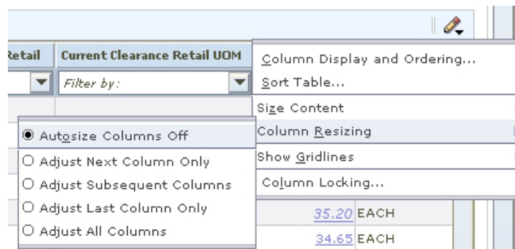
Figure 5–6 Column Resizing
