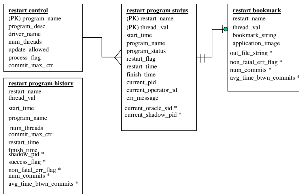
Entity Relationship
