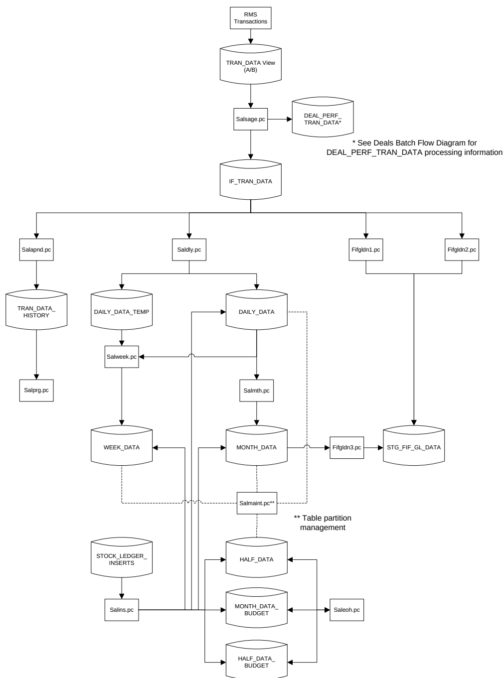
Stock Ledger Data Flow and Batch Modules
