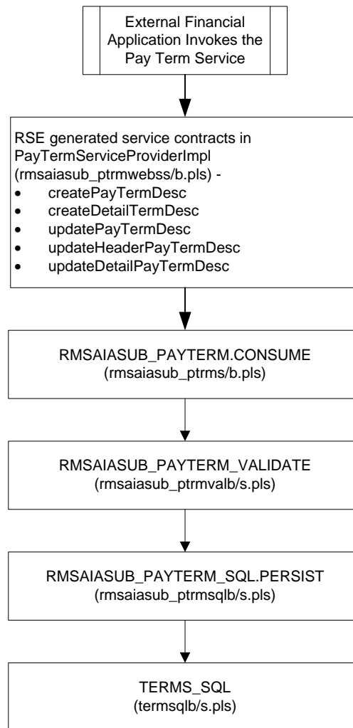
Process Flow for Pay Term Service
