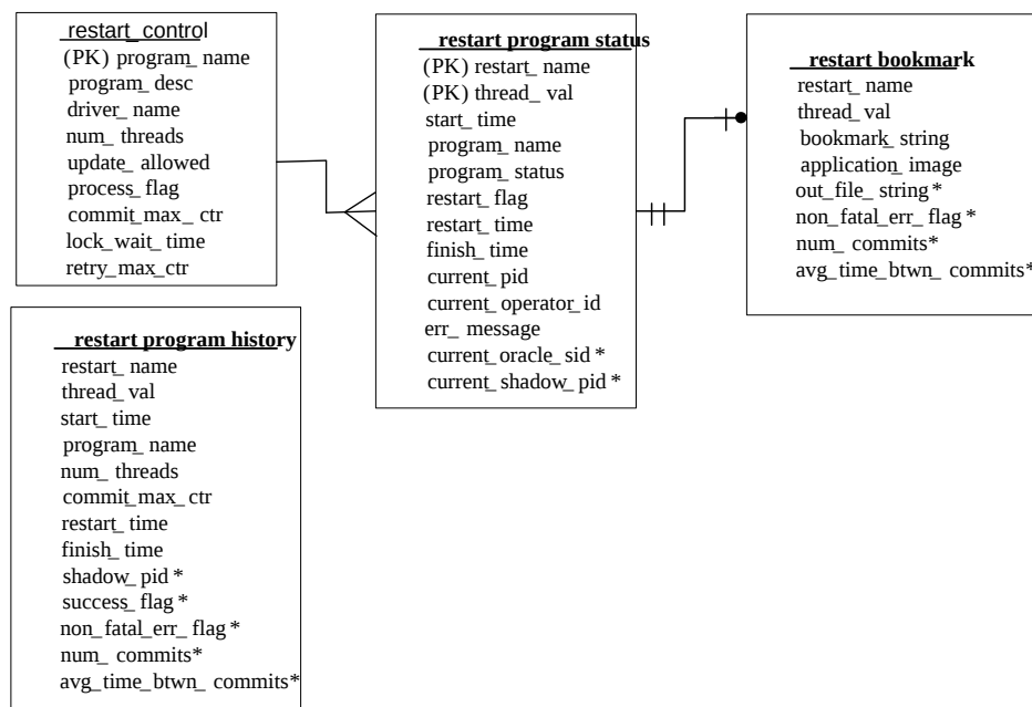
RMS Restart Recovery Entity Relationships Diagram
