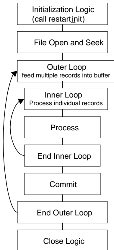
File-based Restart/Recovery Program Flow
