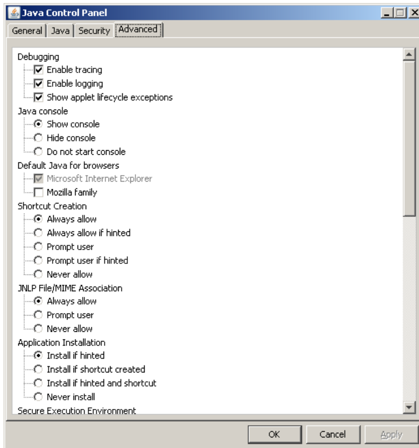
Options in the Advanced Tab
