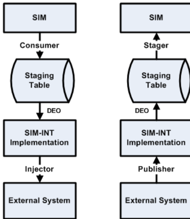
Figure 3-3 SIM RIB Decoupling Framework Overview
