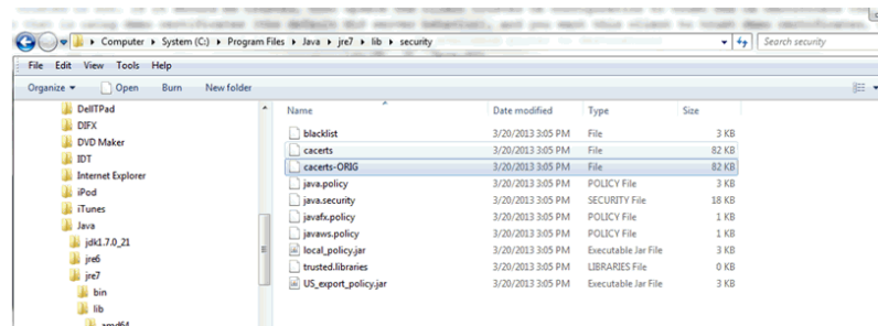
Figure 4-3 Cacert Backup
