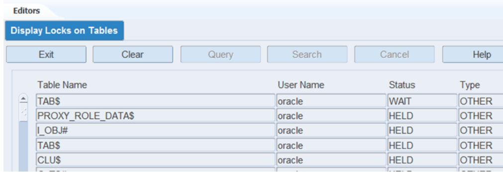
Figure 3–1 Display Locks on Tables Screen
