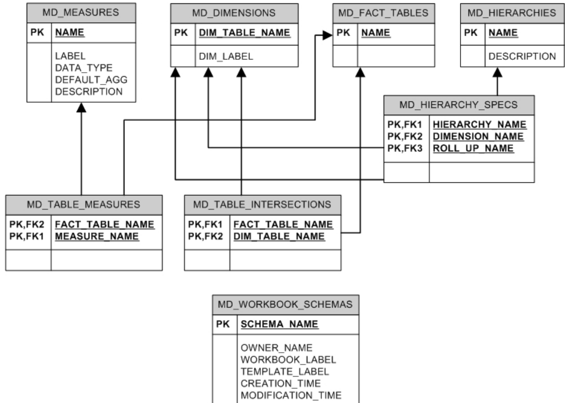
Database Diagram for All Metadata Tables in a Domain or in Each Workbook
