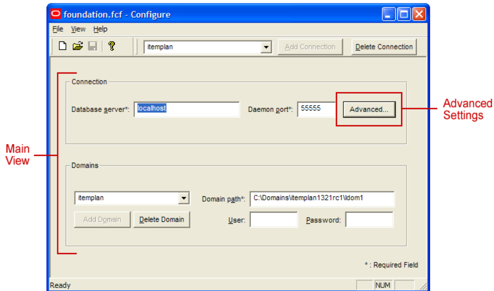
Figure 3–2 eConfigure Utility
