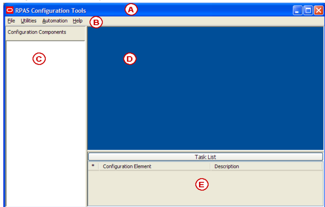
Configuration Tools Window
