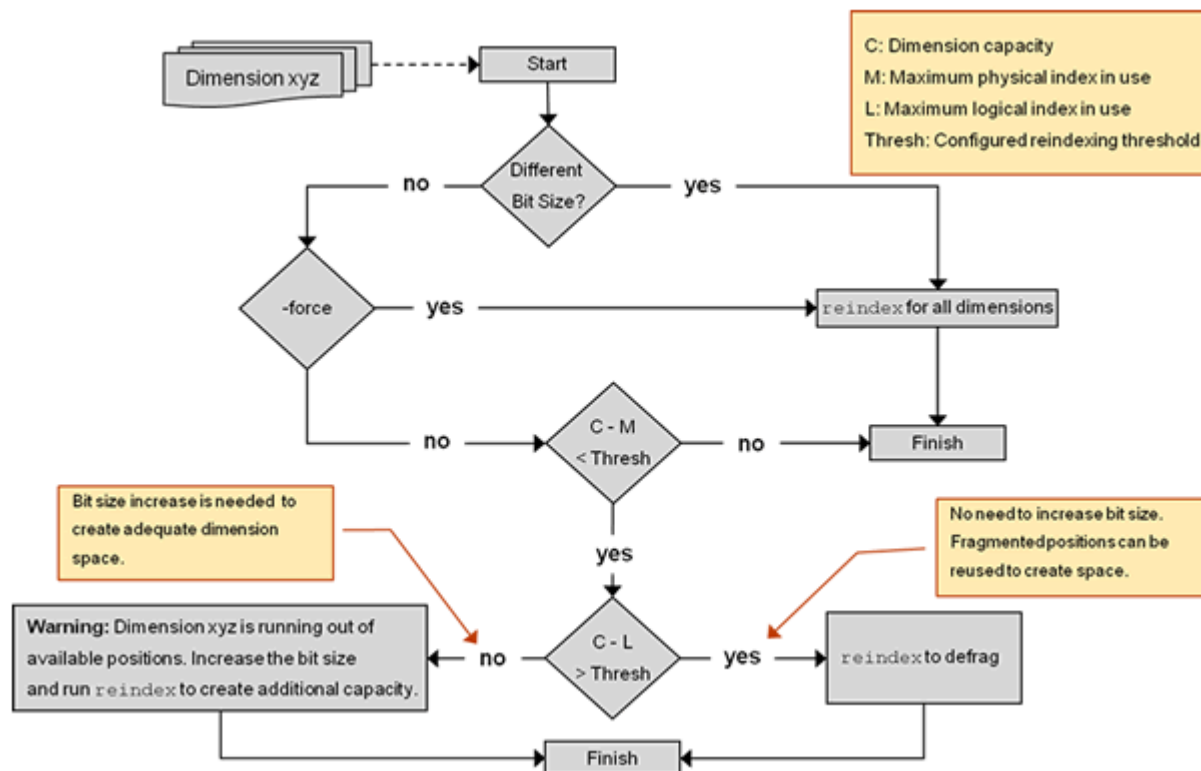
Figure 6–1 Reindexing Domain Process Flow
