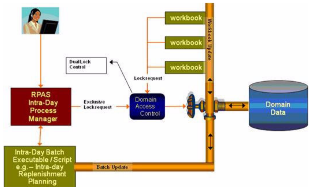
Figure 12–1 Domain Access Control
