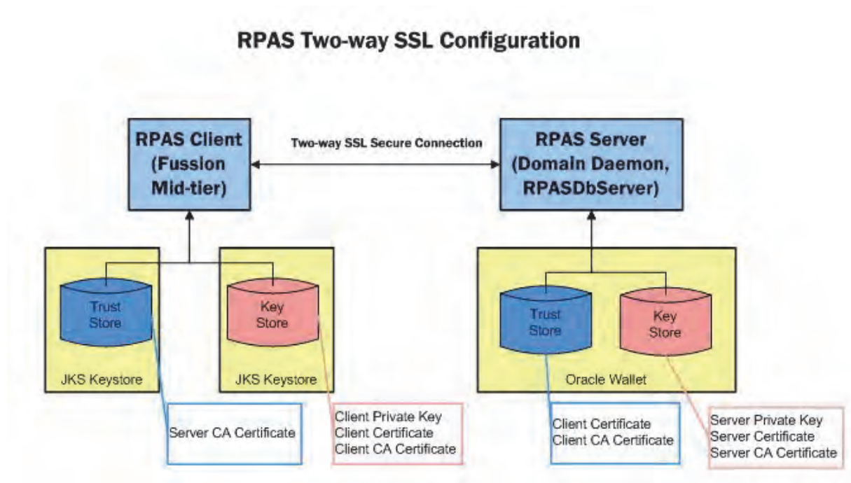
Figure 5-18 Configuration of Two-way SSL for RPAS
