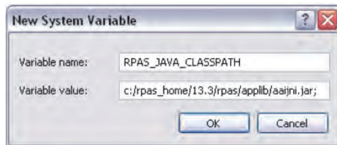
Figure 4-12 Example of RPAS_JAVA_CLASSPATH Variable
