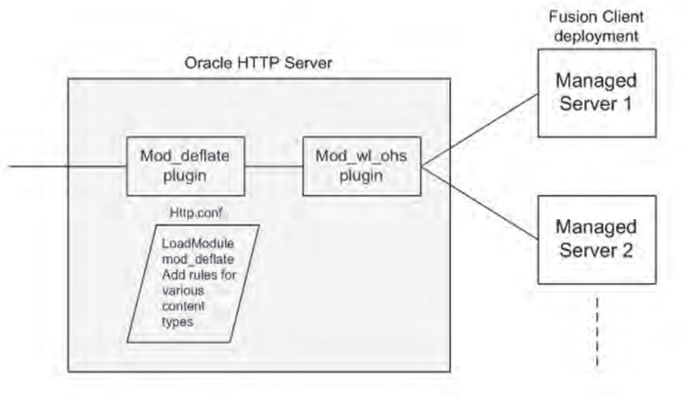
Figure 5–19 Implementing Gzip Compression
