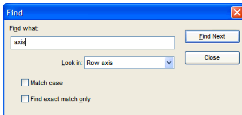
Find Dialog
