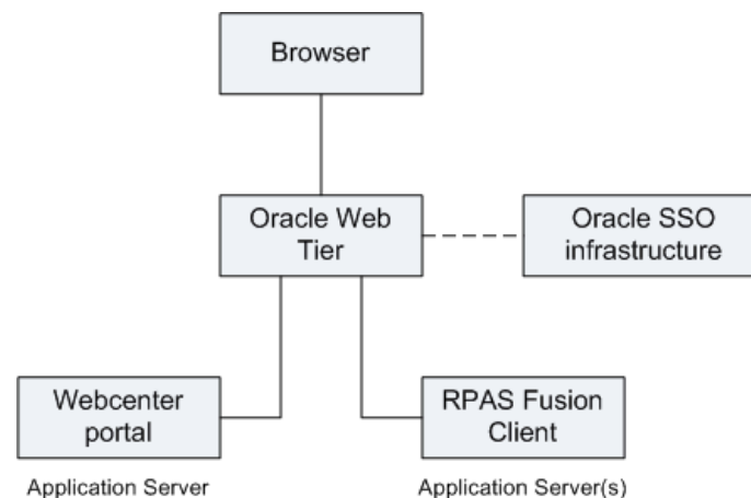
Figure 18–1 OSSO-Based Authentication
