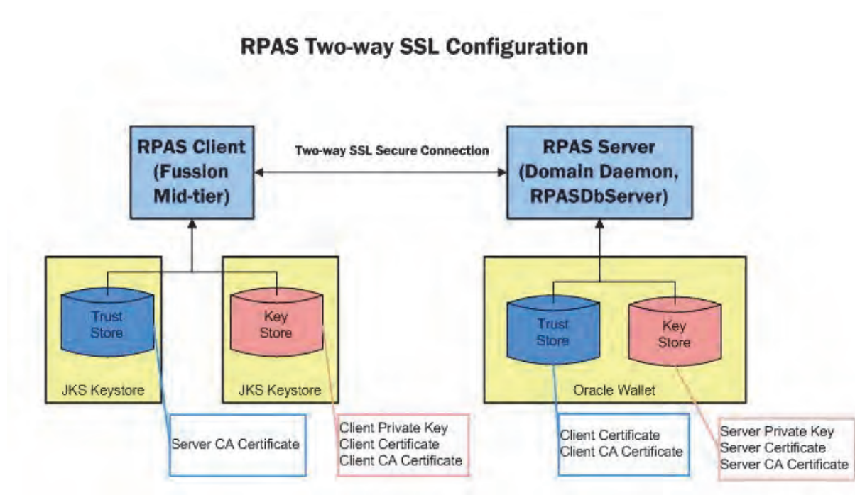
Figure 5–19 Configuration of Two-way SSL for RPAS
