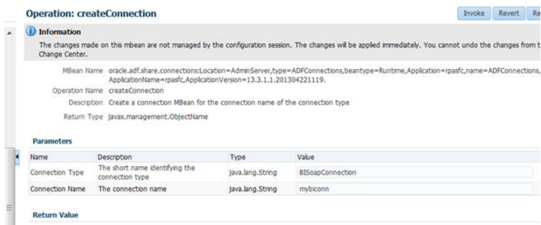
Figure 20–4 Operation: createConnection
