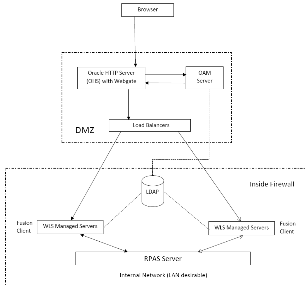
Figure 1–2 Topology for SSO Deployment
