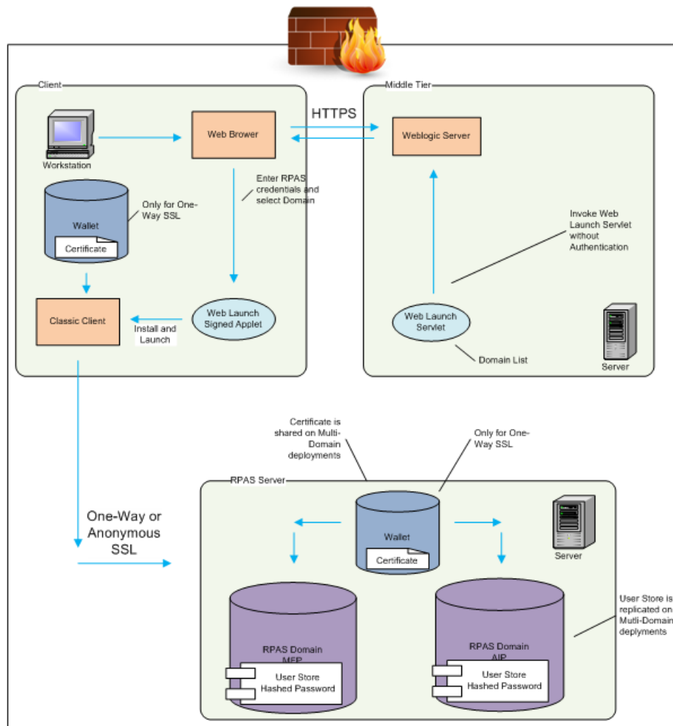
Figure 1–5 Non-SSO Deployment
