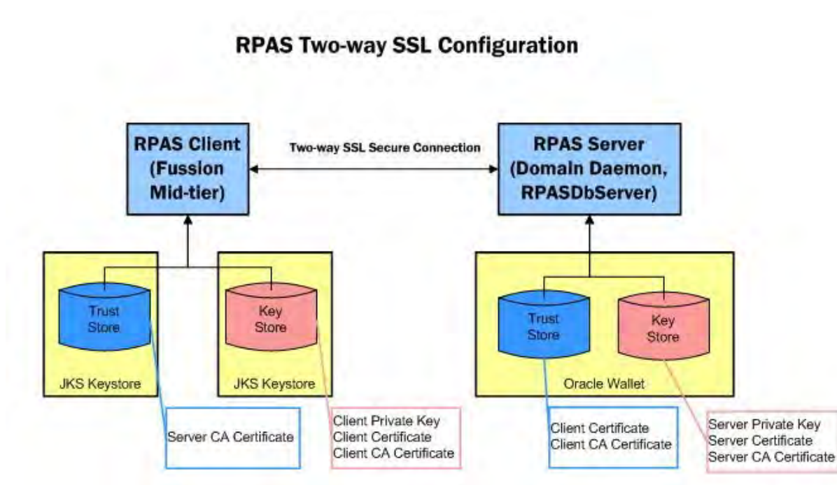
Figure 5-27 Configuration of Two-way SSL for RPAS
