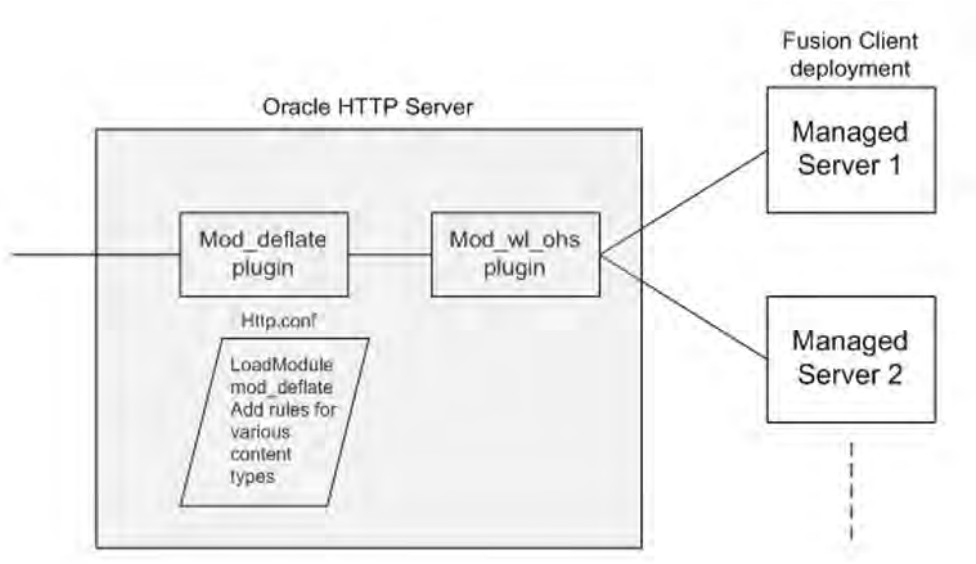
Figure 5-28 Implementing gzip Compression
