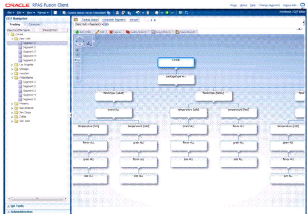
Figure 17–62 Consumer Decision Tree Editor Layout Window
