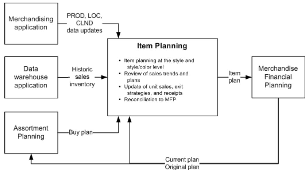
Figure 4–1 Data Flow for the Integration of Item Planning with Other Applications
